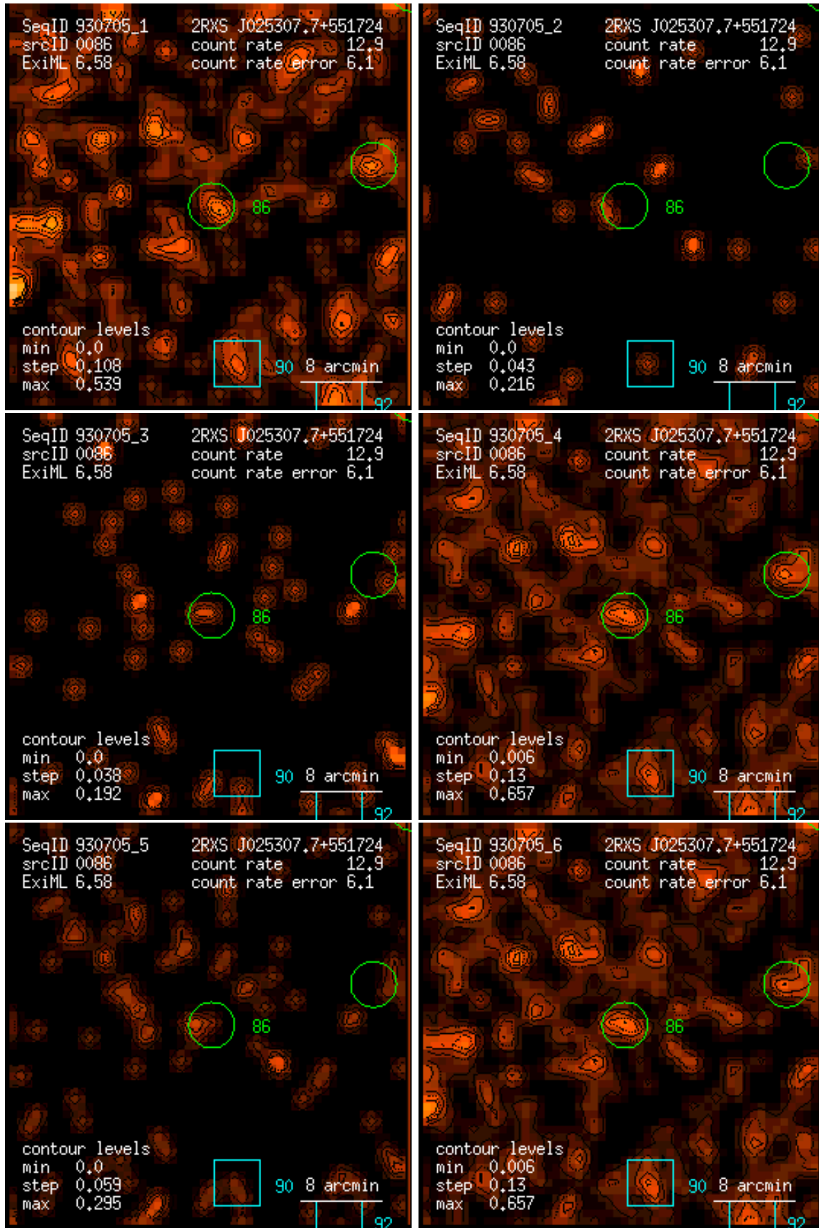
Figure 86: RASS 930705: detection 0086: band rate images, Gaussian filter: (1) PSPC channels 11 – 41, (2) 52 – 90, (3) 91 – 201, (4) 11 – 235, (5) 52 – 201, (6) 11 – 201. Broad band rates in counts/ks. Band rate contour levels in counts/ks/arcmin 2 .
