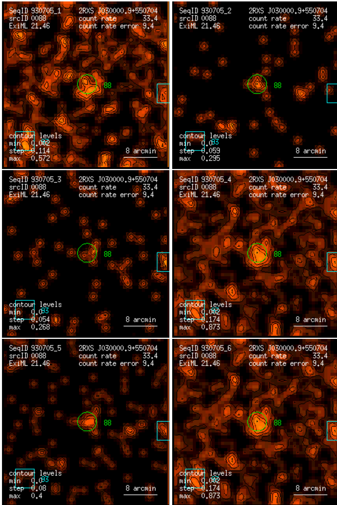
Figure 88: RASS 930705: detection 0088: band rate images, Gaussian filter: (1) PSPC channels 11 – 41, (2) 52 – 90, (3) 91 – 201, (4) 11 – 235, (5) 52 – 201, (6) 11 – 201. Broad band rates in counts/ks. Band rate contour levels in counts/ks/arcmin 2 .
