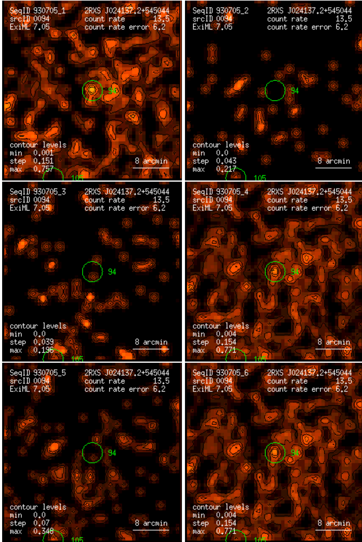
Figure 94: RASS 930705: detection 0094: band rate images, Gaussian filter: (1) PSPC channels 11 – 41, (2) 52 – 90, (3) 91 – 201, (4) 11 – 235, (5) 52 – 201, (6) 11 – 201. Broad band rates in counts/ks. Band rate contour levels in counts/ks/arcmin 2 .
