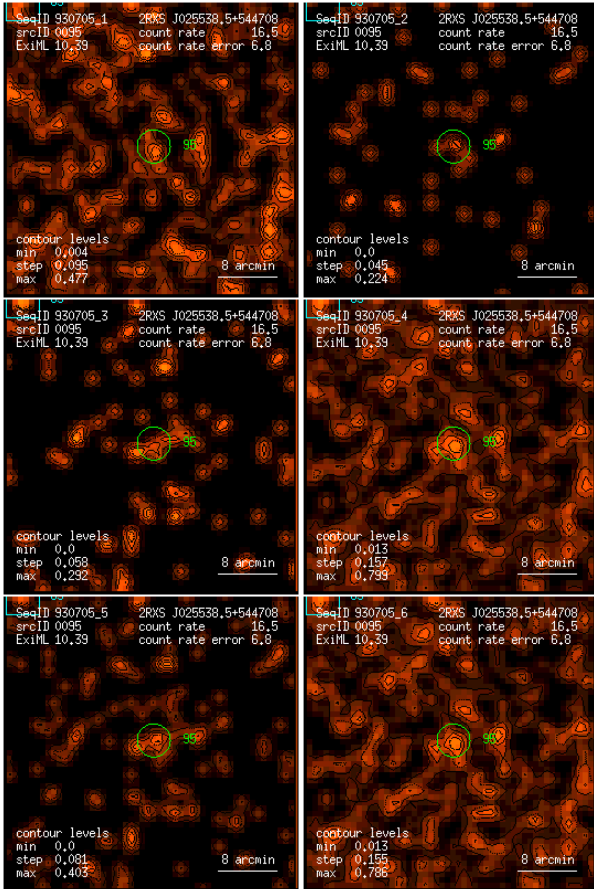
Figure 95: RASS 930705: detection 0095: band rate images, Gaussian filter: (1) PSPC channels 11 – 41, (2) 52 – 90, (3) 91 – 201, (4) 11 – 235, (5) 52 – 201, (6) 11 – 201. Broad band rates in counts/ks. Band rate contour levels in counts/ks/arcmin 2 .
