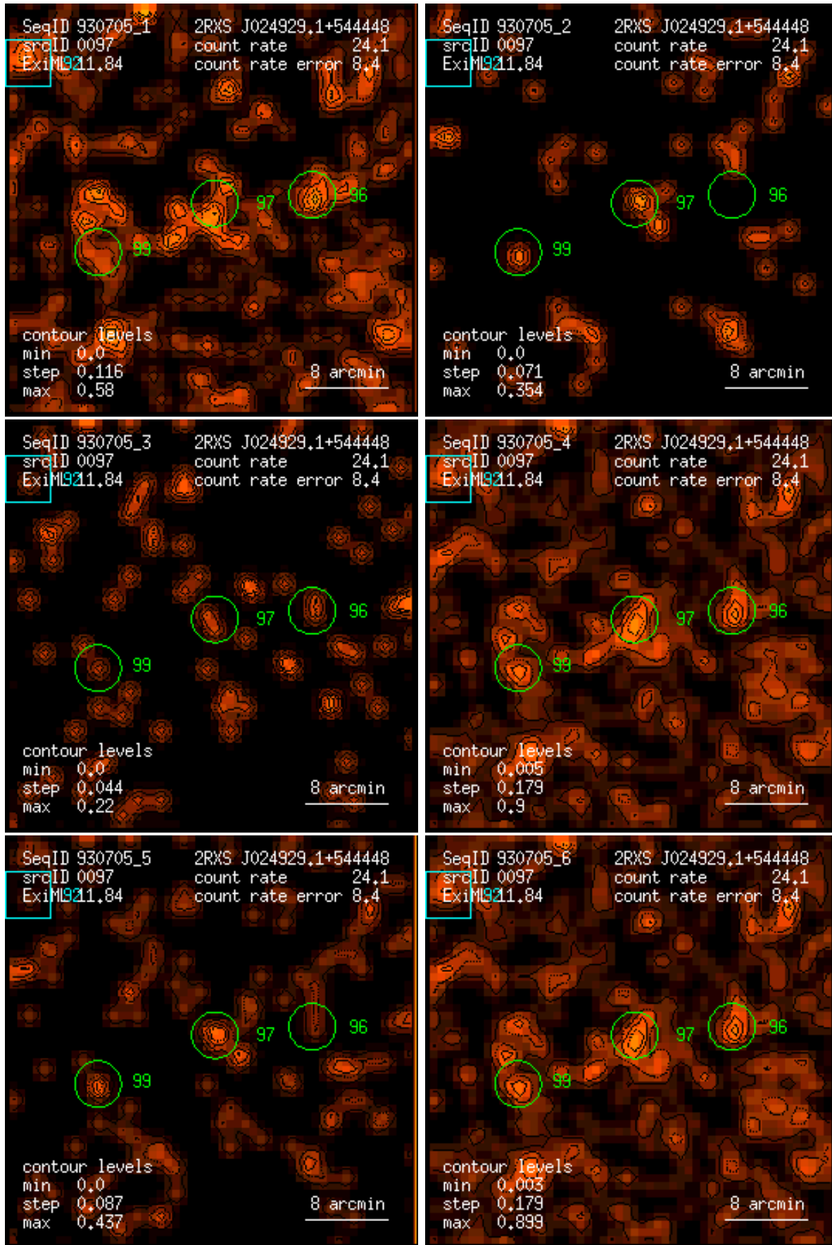
Figure 97: RASS 930705: detection 0097: band rate images, Gaussian filter: (1) PSPC channels 11 – 41, (2) 52 – 90, (3) 91 – 201, (4) 11 – 235, (5) 52 – 201, (6) 11 – 201. Broad band rates in counts/ks. Band rate contour levels in counts/ks/arcmin 2 .
