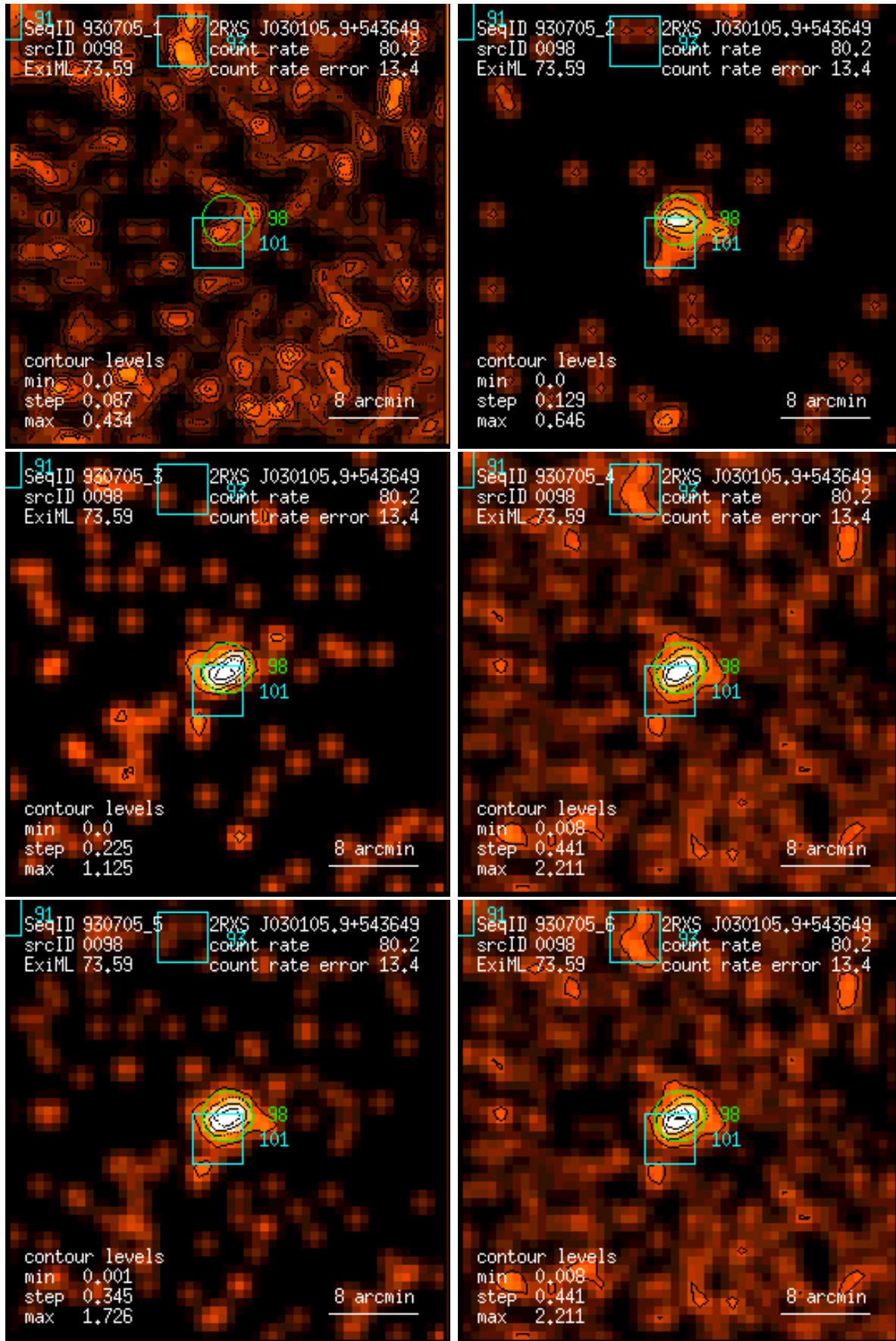
Figure 98: RASS 930705: detection 0098: band rate images, Gaussian filter: (1) PSPC channels 11 – 41, (2) 52 – 90, (3) 91 – 201, (4) 11 – 235, (5) 52 – 201, (6) 11 – 201. Broad band rates in counts/ks. Band rate contour levels in counts/ks/arcmin 2 .
