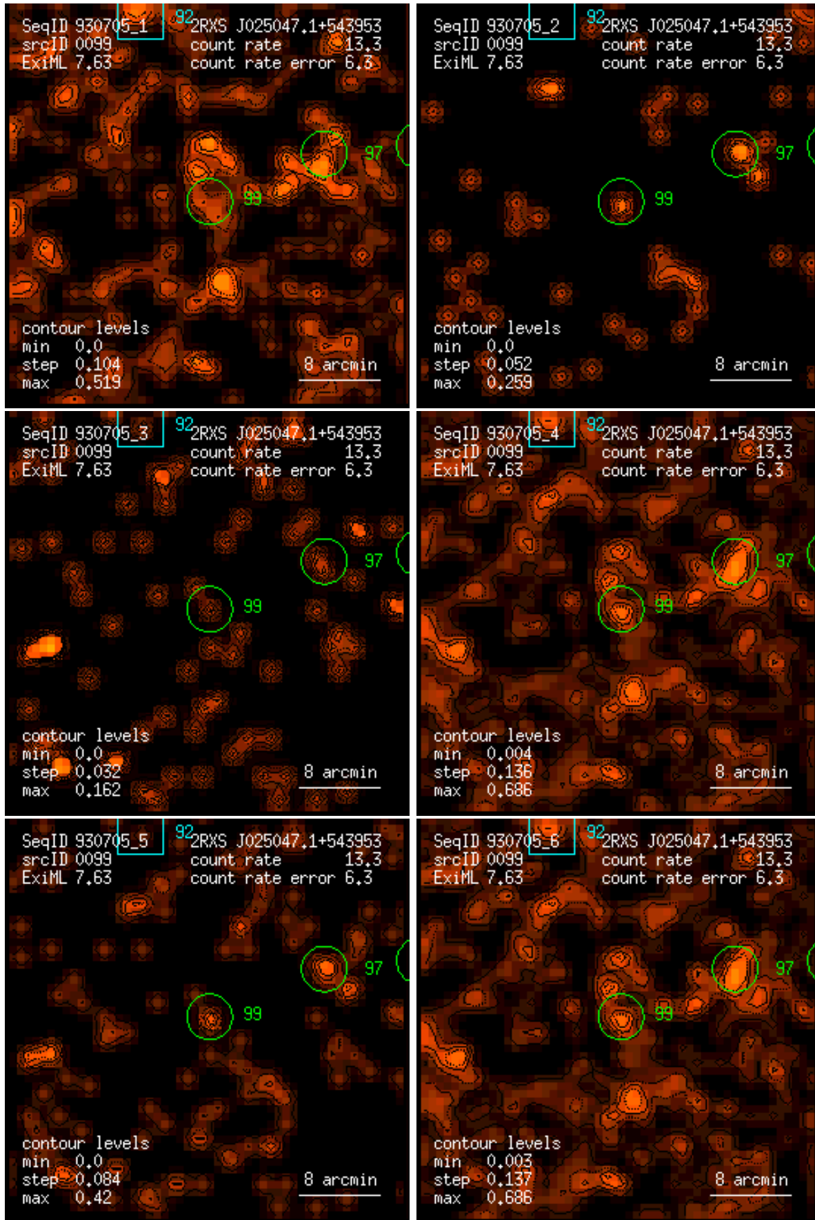
Figure 99: RASS 930705: detection 0099: band rate images, Gaussian filter: (1) PSPC channels 11 – 41, (2) 52 – 90, (3) 91 – 201, (4) 11 – 235, (5) 52 – 201, (6) 11 – 201. Broad band rates in counts/ks. Band rate contour levels in counts/ks/arcmin 2 .
