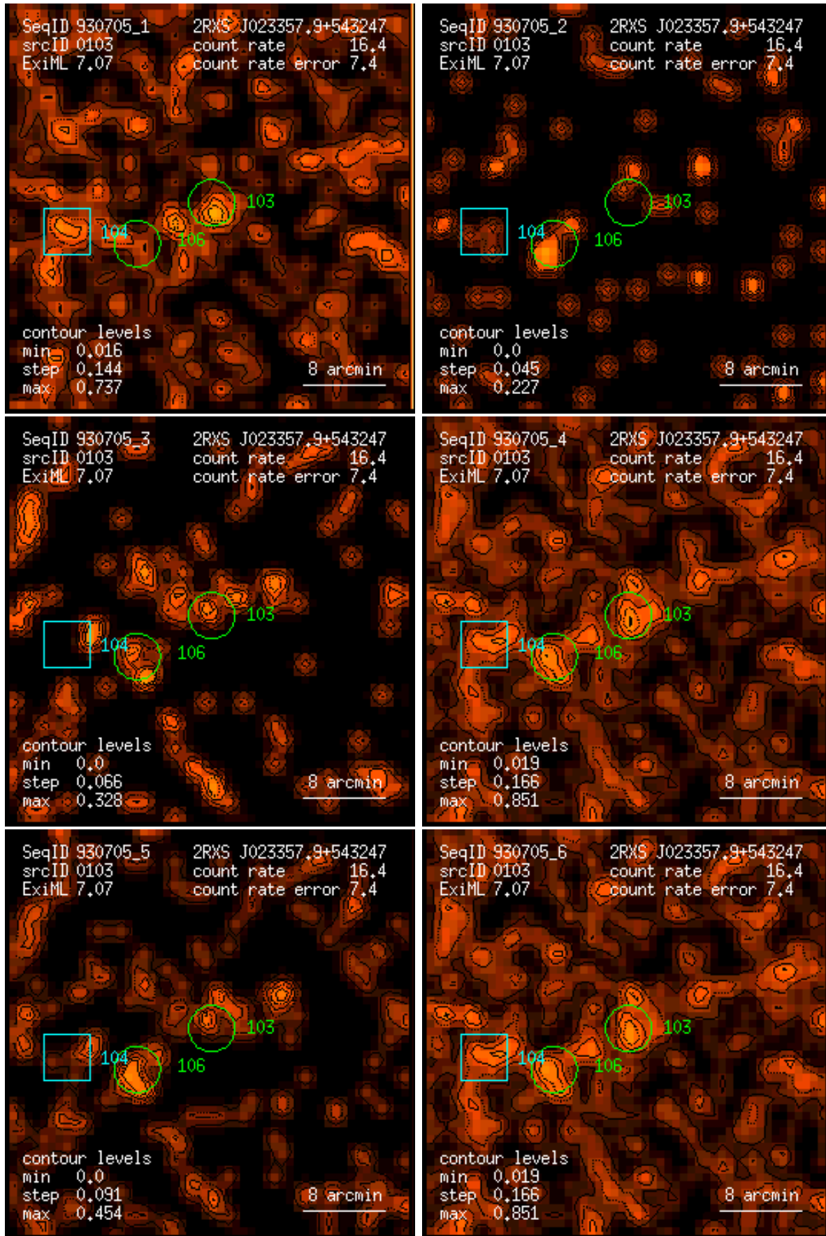
Figure 103: RASS 930705: detection 0103: band rate images, Gaussian filter: (1) PSPC channels 11 – 41, (2) 52 – 90, (3) 91 – 201, (4) 11 – 235, (5) 52 – 201, (6) 11 – 201. Broad band rates in counts/ks. Band rate contour levels in counts/ks/arcmin 2 .
