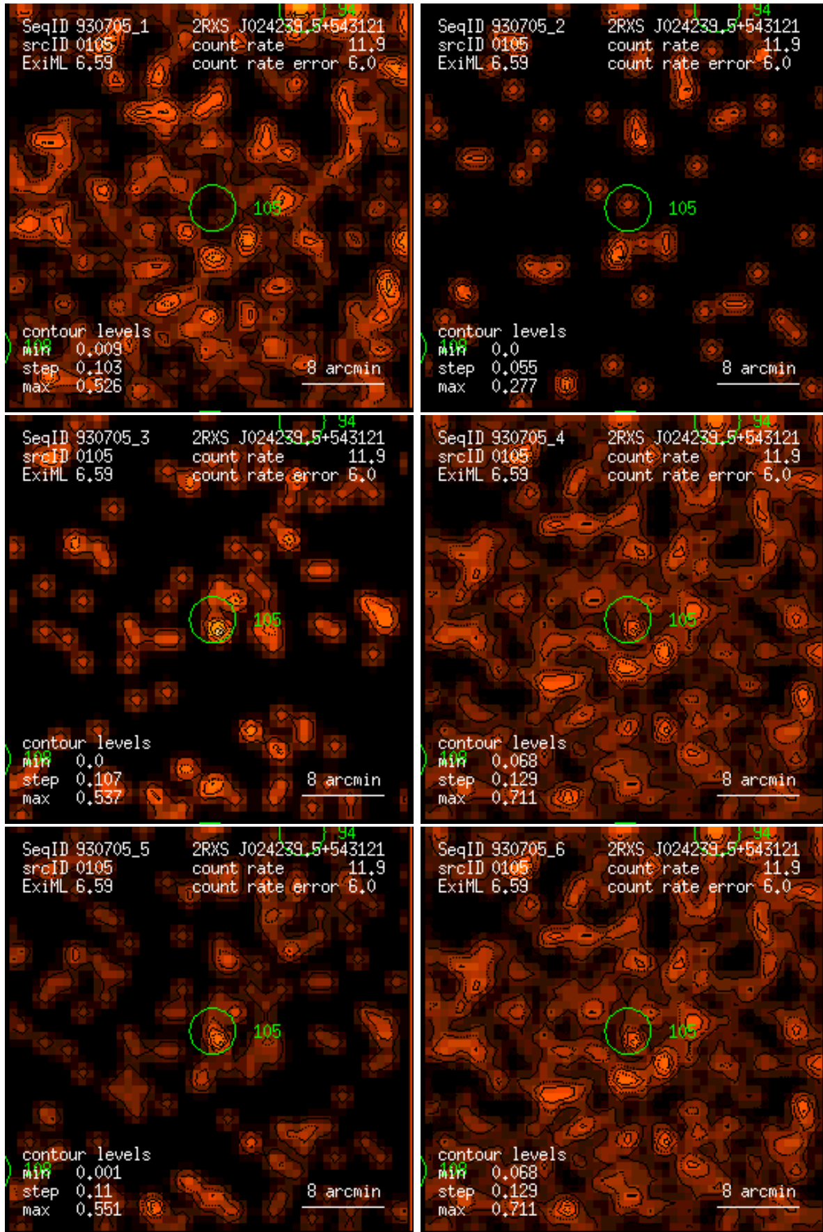
Figure 105: RASS 930705: detection 0105: band rate images, Gaussian filter: (1) PSPC channels 11 – 41, (2) 52 – 90, (3) 91 – 201, (4) 11 – 235, (5) 52 – 201, (6) 11 – 201. Broad band rates in counts/ks. Band rate contour levels in counts/ks/arcmin 2 .
