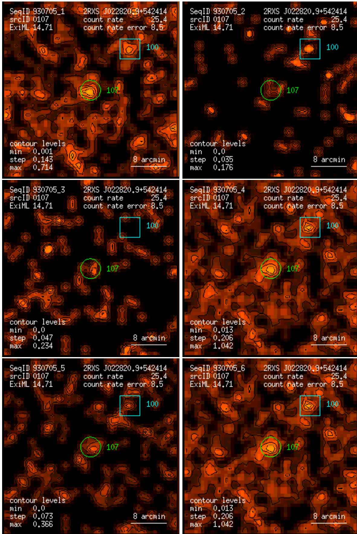
Figure 107: RASS 930705: detection 0107: band rate images, Gaussian filter: (1) PSPC channels 11 – 41, (2) 52 – 90, (3) 91 – 201, (4) 11 – 235, (5) 52 – 201, (6) 11 – 201. Broad band rates in counts/ks. Band rate contour levels in counts/ks/arcmin 2 .
