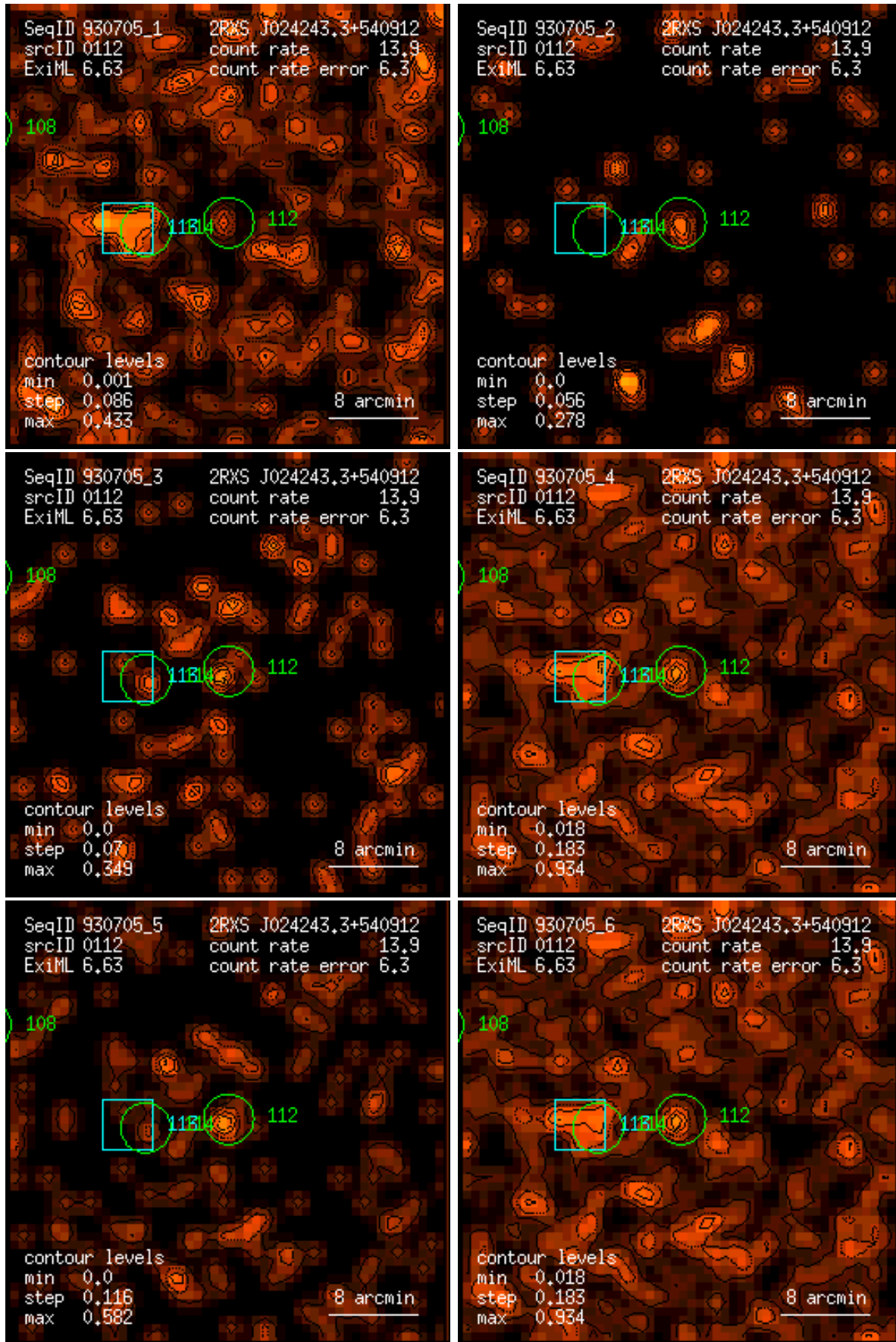
Figure 112: RASS 930705: detection 0112: band rate images, Gaussian filter: (1) PSPC channels 11 – 41, (2) 52 – 90, (3) 91 – 201, (4) 11 – 235, (5) 52 – 201, (6) 11 – 201. Broad band rates in counts/ks. Band rate contour levels in counts/ks/arcmin 2 .
