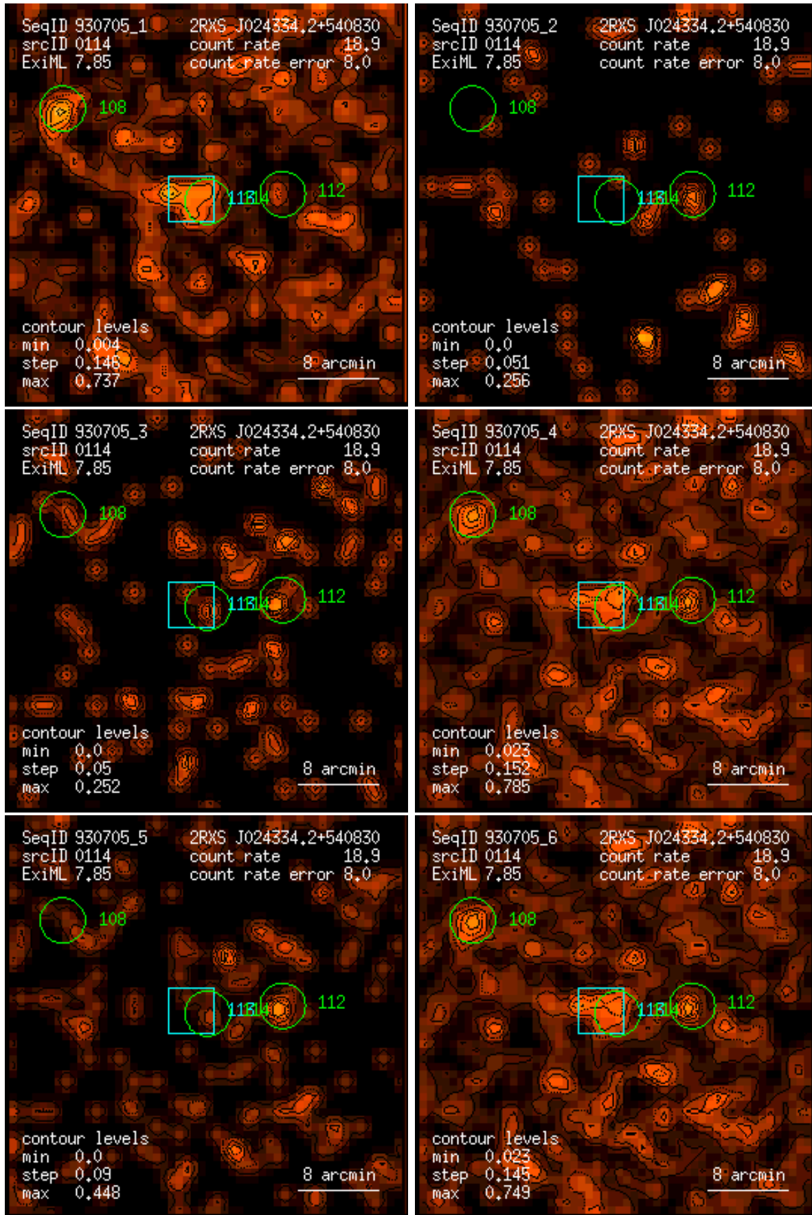
Figure 114: RASS 930705: detection 0114: band rate images, Gaussian filter: (1) PSPC channels 11 – 41, (2) 52 – 90, (3) 91 – 201, (4) 11 – 235, (5) 52 – 201, (6) 11 – 201. Broad band rates in counts/ks. Band rate contour levels in counts/ks/arcmin 2 .
