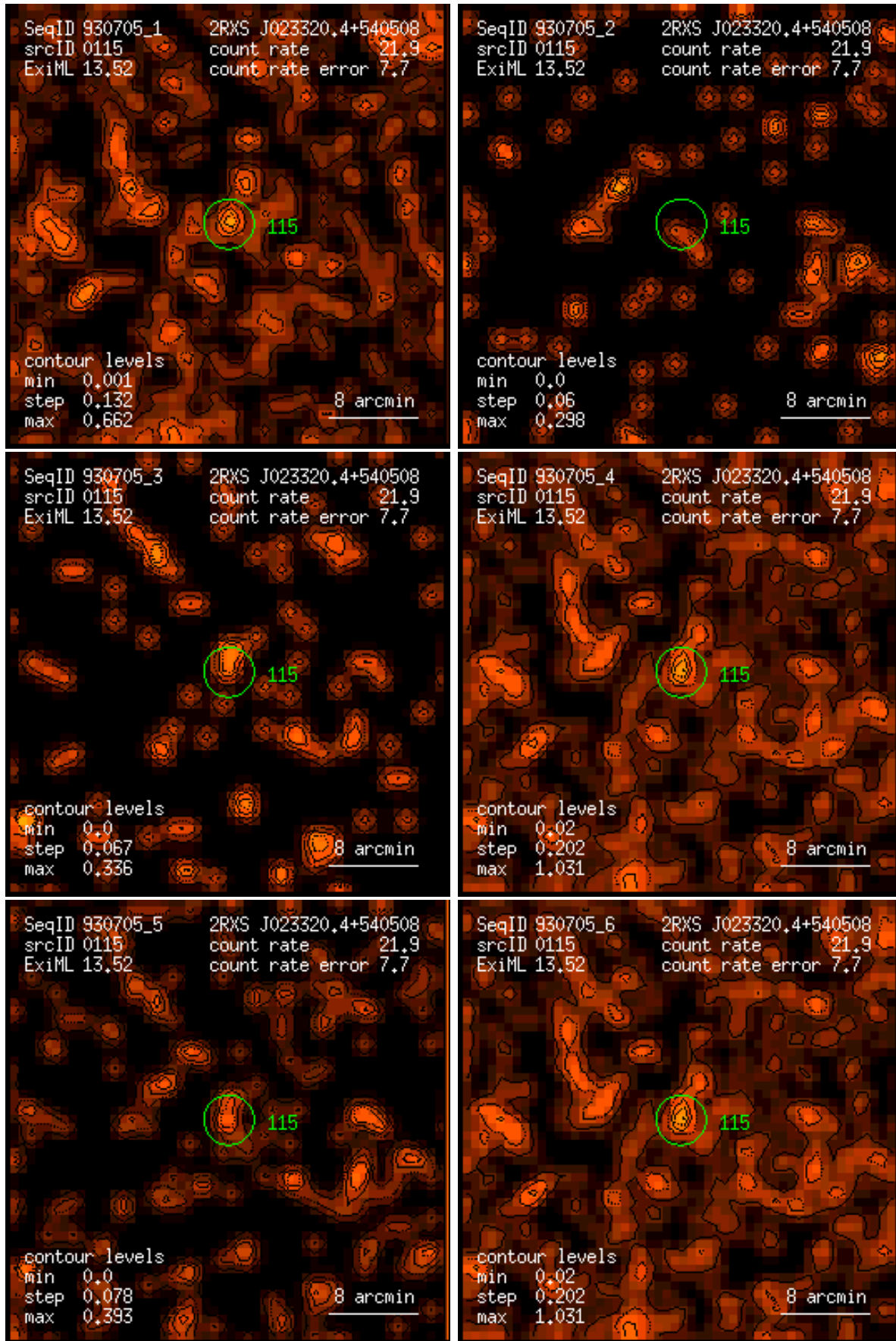
Figure 115: RASS 930705: detection 0115: band rate images, Gaussian filter: (1) PSPC channels 11 – 41, (2) 52 – 90, (3) 91 – 201, (4) 11 – 235, (5) 52 – 201, (6) 11 – 201. Broad band rates in counts/ks. Band rate contour levels in counts/ks/arcmin 2 .
