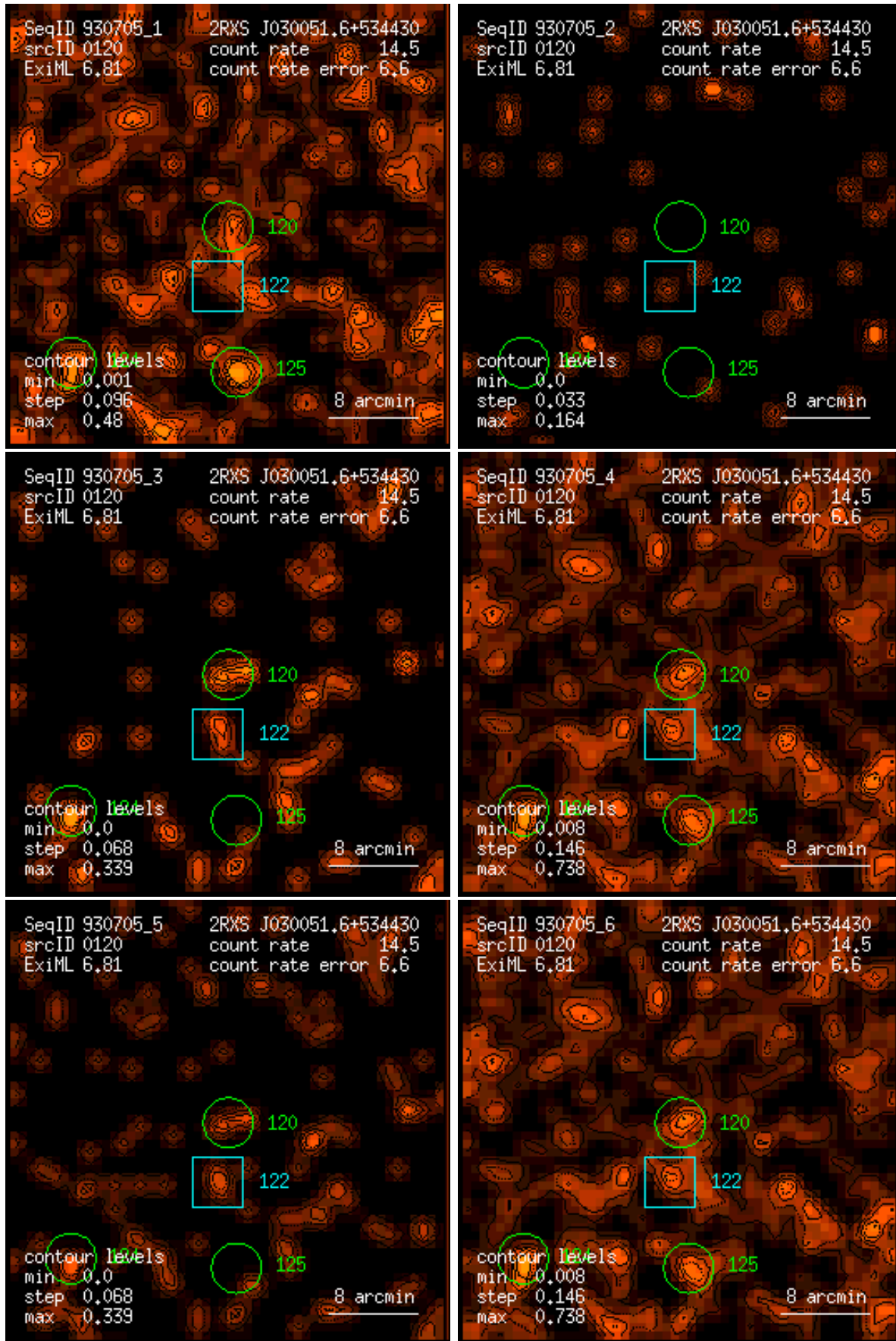
Figure 120: RASS 930705: detection 0120: band rate images, Gaussian filter: (1) PSPC channels 11 – 41, (2) 52 – 90, (3) 91 – 201, (4) 11 – 235, (5) 52 – 201, (6) 11 – 201. Broad band rates in counts/ks. Band rate contour levels in counts/ks/arcmin 2 .
