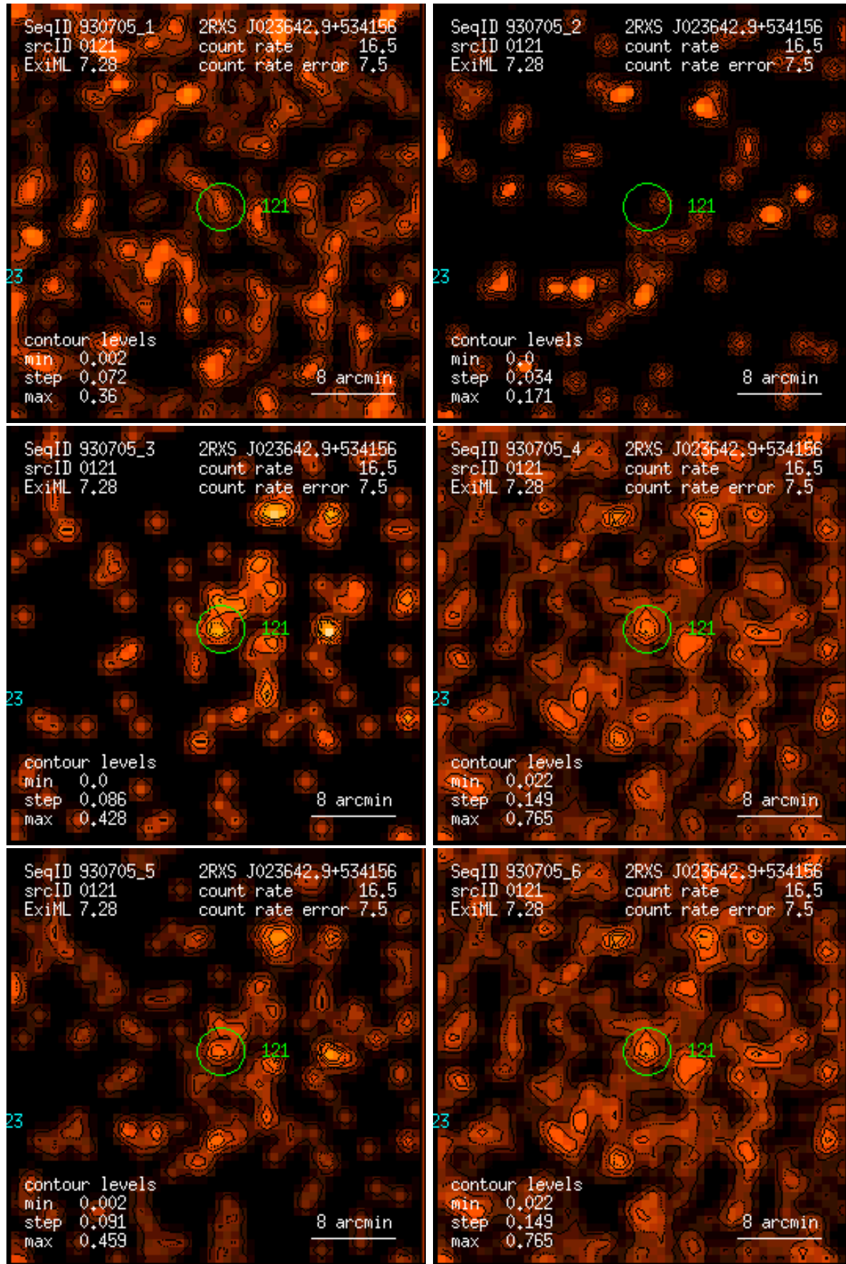
Figure 121: RASS 930705: detection 0121: band rate images, Gaussian filter: (1) PSPC channels 11 – 41, (2) 52 – 90, (3) 91 – 201, (4) 11 – 235, (5) 52 – 201, (6) 11 – 201. Broad band rates in counts/ks. Band rate contour levels in counts/ks/arcmin 2 .
