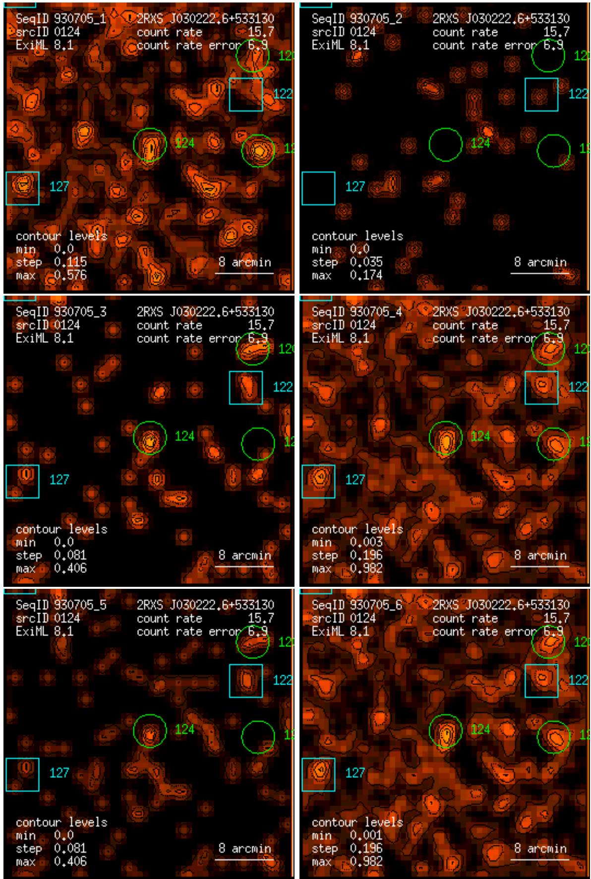
Figure 124: RASS 930705: detection 0124: band rate images, Gaussian filter: (1) PSPC channels 11 – 41, (2) 52 – 90, (3) 91 – 201, (4) 11 – 235, (5) 52 – 201, (6) 11 – 201. Broad band rates in counts/ks. Band rate contour levels in counts/ks/arcmin 2 .
