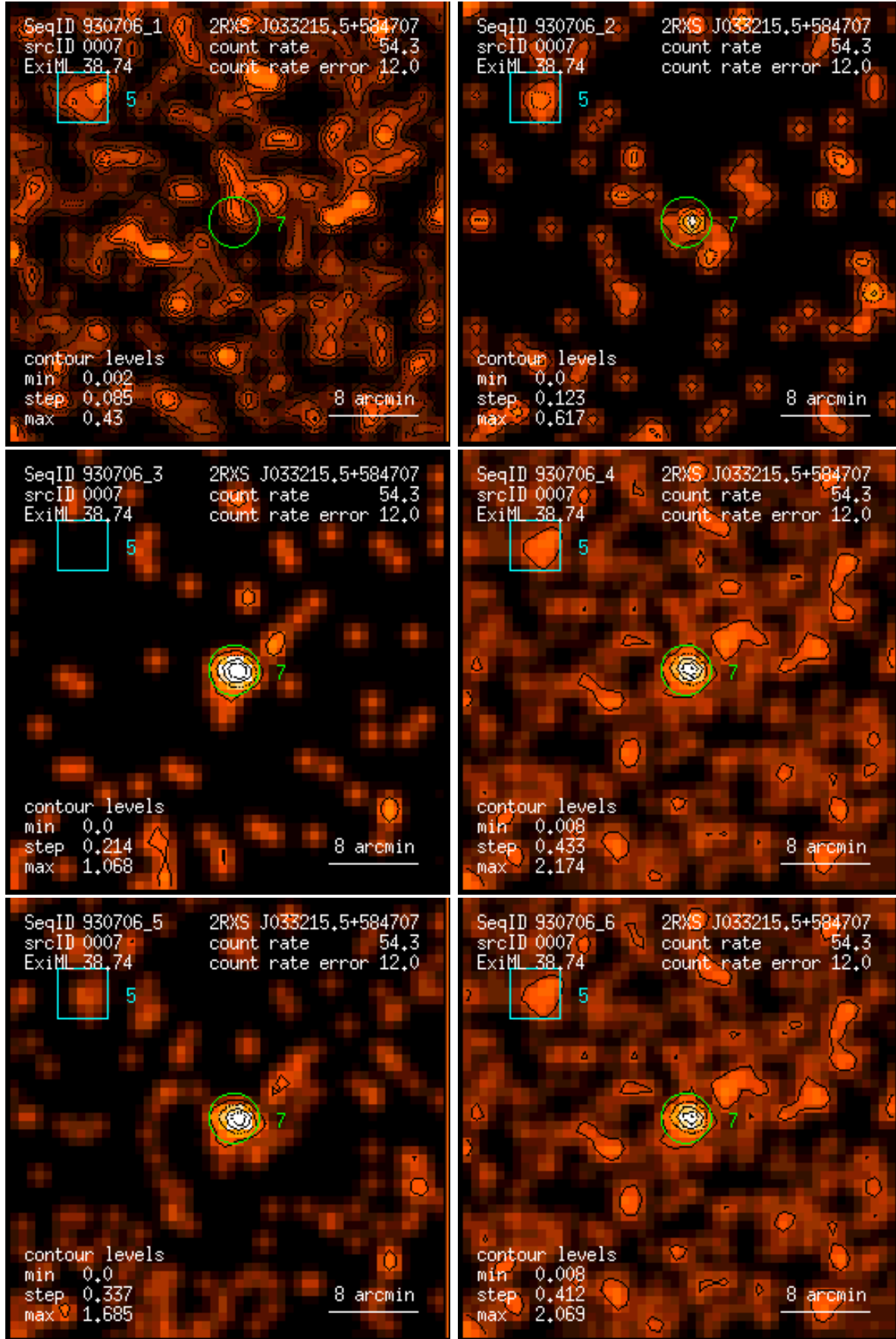
Figure 7: RASS 930706: detection 0007: band rate images, Gaussian filter: (1) PSPC channels 11 – 41, (2) 52 – 90, (3) 91 – 201, (4) 11 – 235, (5) 52 – 201, (6) 11 – 201. Broad band rates in counts/ks. Band rate contour levels in counts/ks/arcmin 2 .
