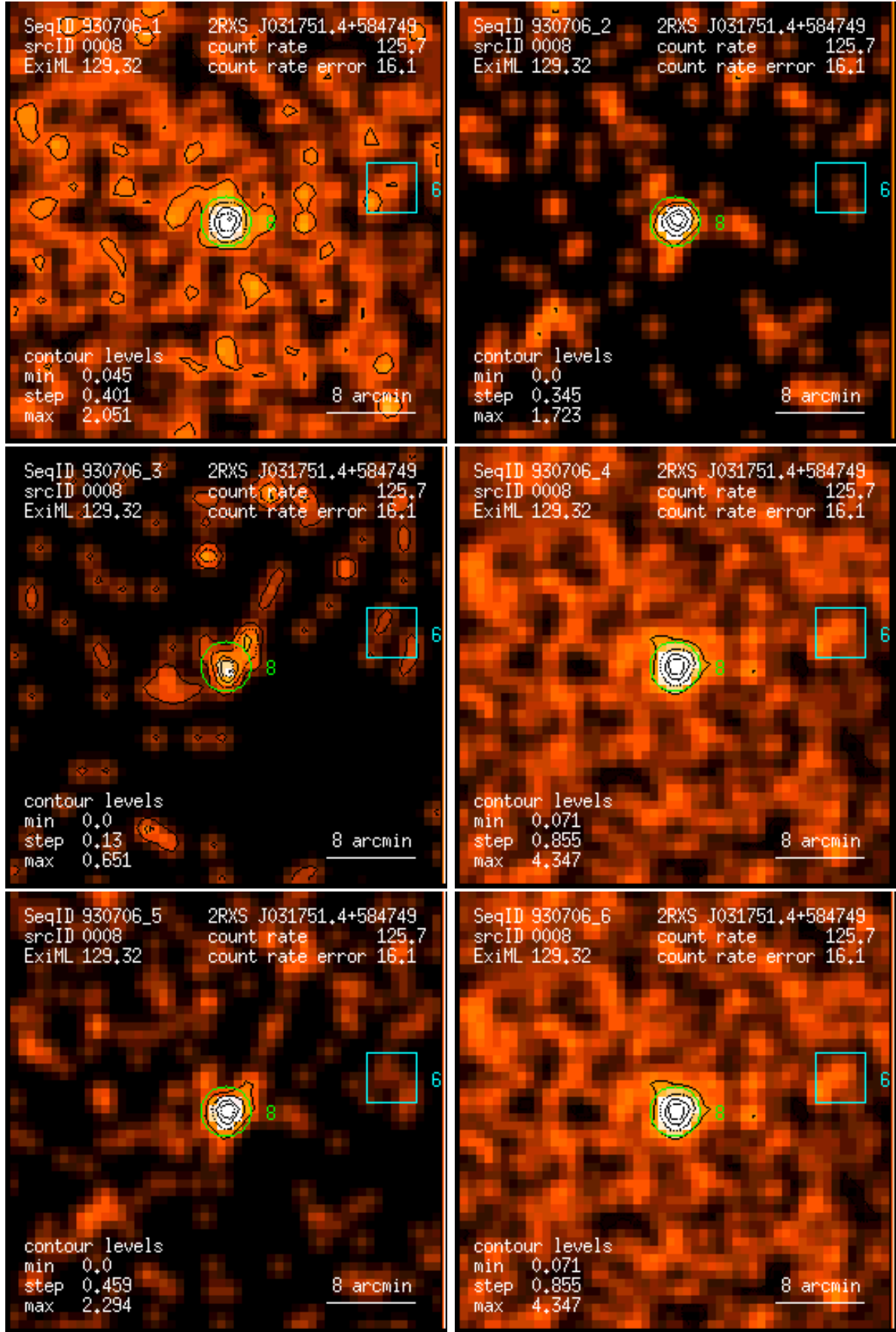
Figure 8: RASS 930706: detection 0008: band rate images, Gaussian filter: (1) PSPC channels 11 – 41, (2) 52 – 90, (3) 91 – 201, (4) 11 – 235, (5) 52 – 201, (6) 11 – 201. Broad band rates in counts/ks. Band rate contour levels in counts/ks/arcmin 2 .
