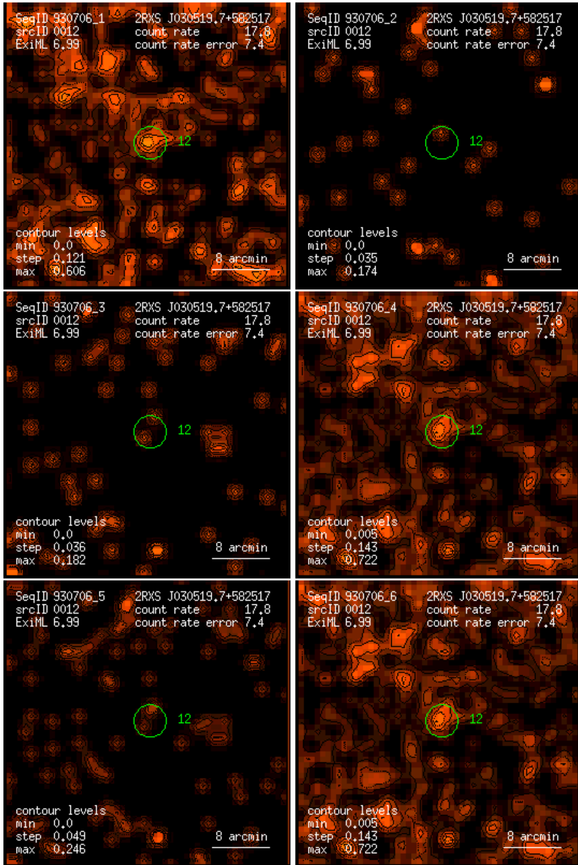
Figure 12: RASS 930706: detection 0012: band rate images, Gaussian filter: (1) PSPC channels 11 – 41, (2) 52 – 90, (3) 91 – 201, (4) 11 – 235, (5) 52 – 201, (6) 11 – 201. Broad band rates in counts/ks. Band rate contour levels in counts/ks/arcmin 2 .
