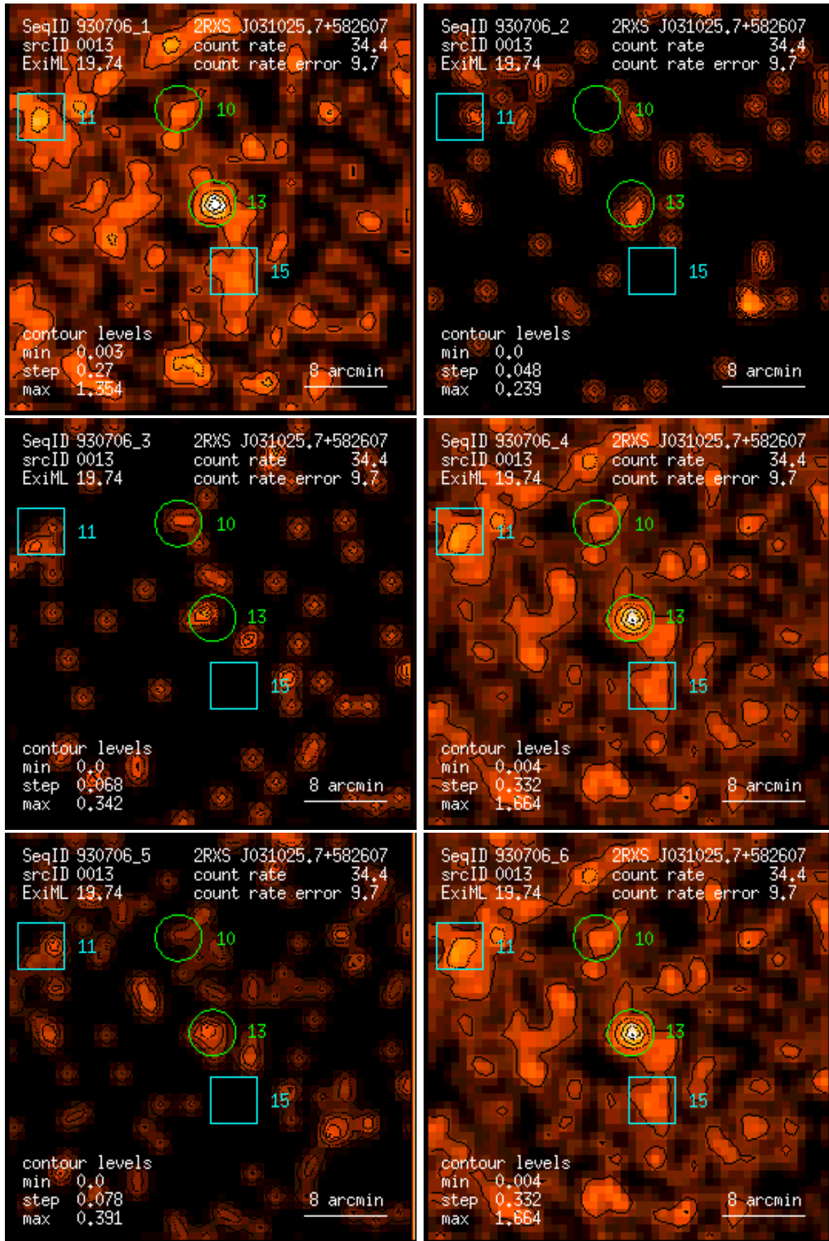
Figure 13: RASS 930706: detection 0013: band rate images, Gaussian filter: (1) PSPC channels 11 – 41, (2) 52 – 90, (3) 91 – 201, (4) 11 – 235, (5) 52 – 201, (6) 11 – 201. Broad band rates in counts/ks. Band rate contour levels in counts/ks/arcmin 2 .
