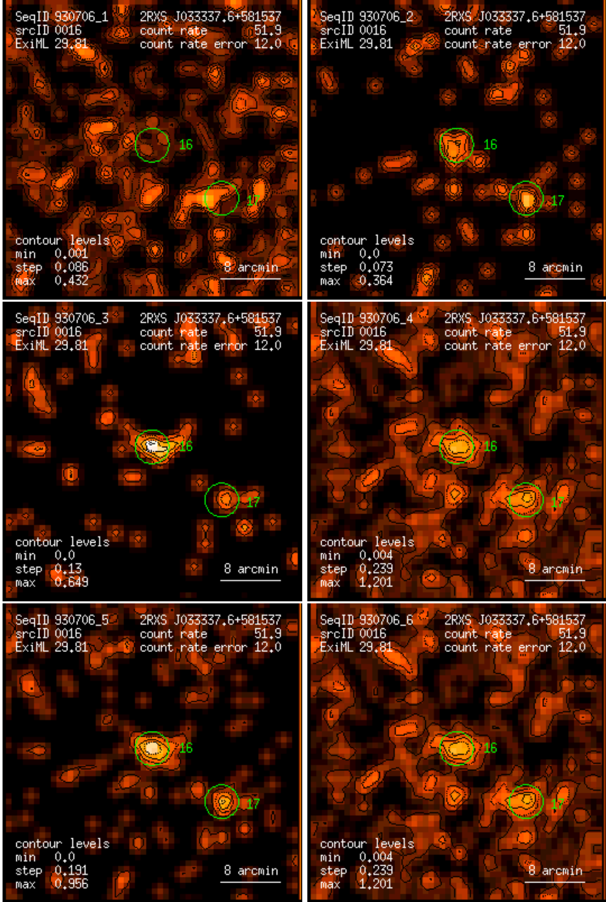
Figure 16: RASS 930706: detection 0016: band rate images, Gaussian filter: (1) PSPC channels 11 – 41, (2) 52 – 90, (3) 91 – 201, (4) 11 – 235, (5) 52 – 201, (6) 11 – 201. Broad band rates in counts/ks. Band rate contour levels in counts/ks/arcmin 2 .
