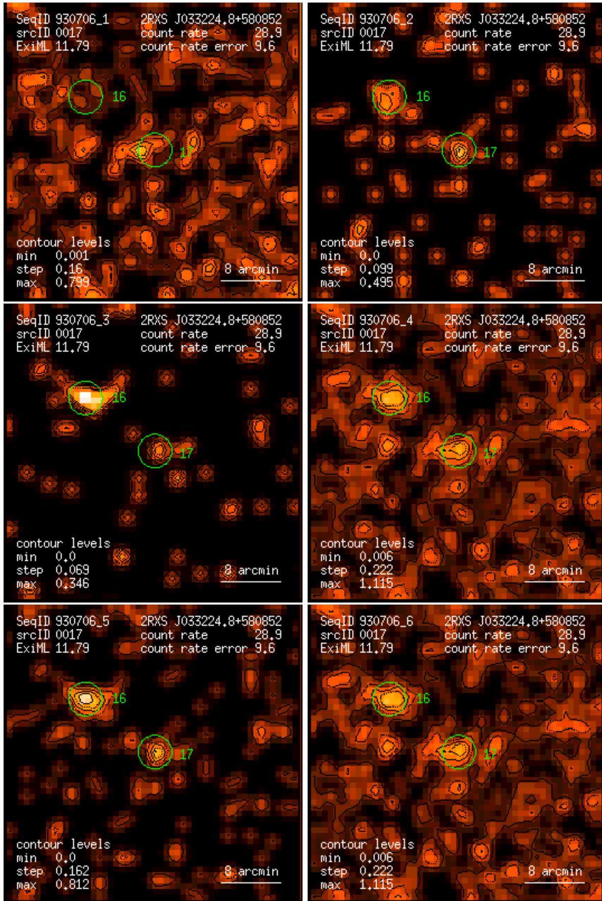
Figure 17: RASS 930706: detection 0017: band rate images, Gaussian filter: (1) PSPC channels 11 – 41, (2) 52 – 90, (3) 91 – 201, (4) 11 – 235, (5) 52 – 201, (6) 11 – 201. Broad band rates in counts/ks. Band rate contour levels in counts/ks/arcmin 2 .
