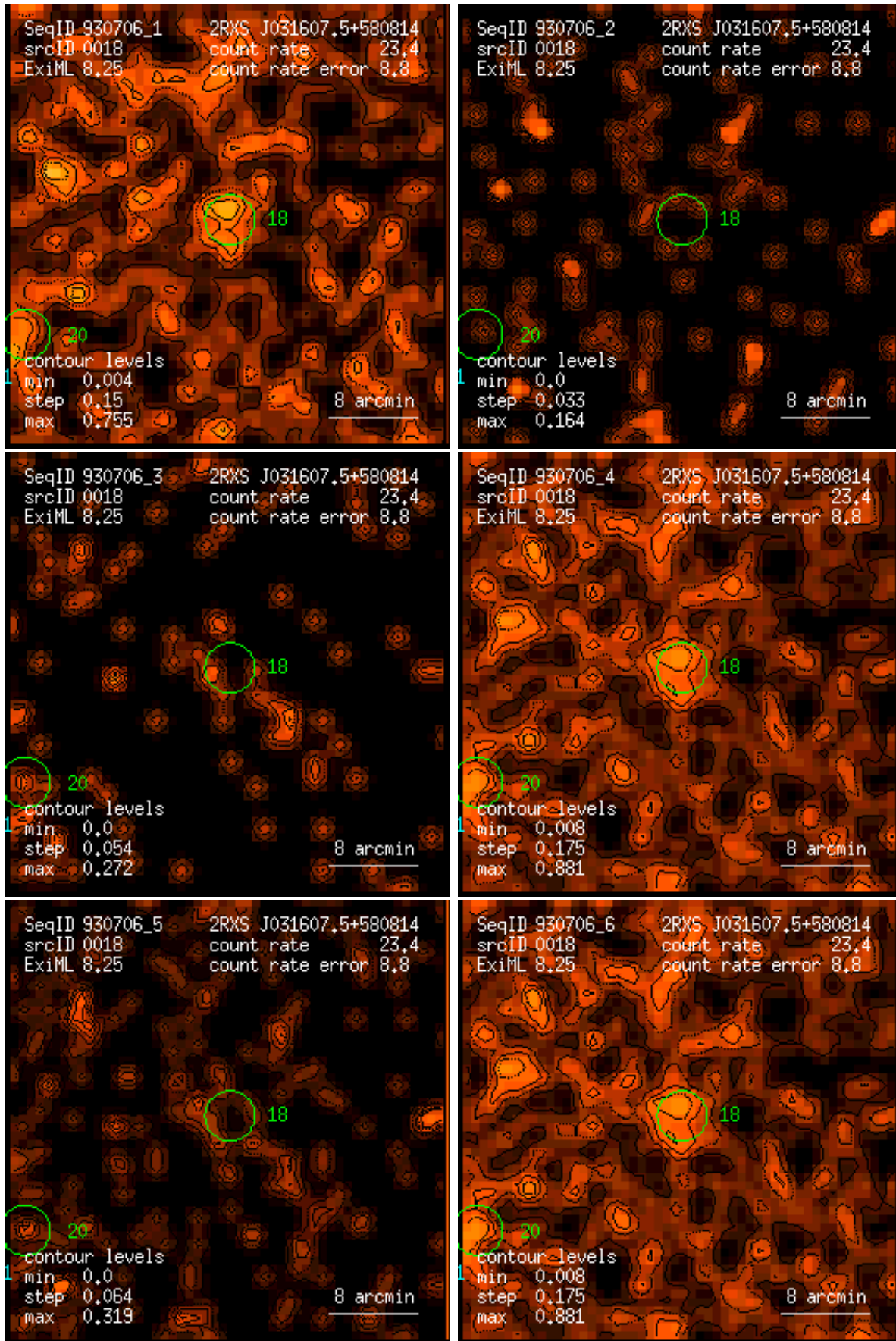
Figure 18: RASS 930706: detection 0018: band rate images, Gaussian filter: (1) PSPC channels 11 – 41, (2) 52 – 90, (3) 91 – 201, (4) 11 – 235, (5) 52 – 201, (6) 11 – 201. Broad band rates in counts/ks. Band rate contour levels in counts/ks/arcmin 2 .
