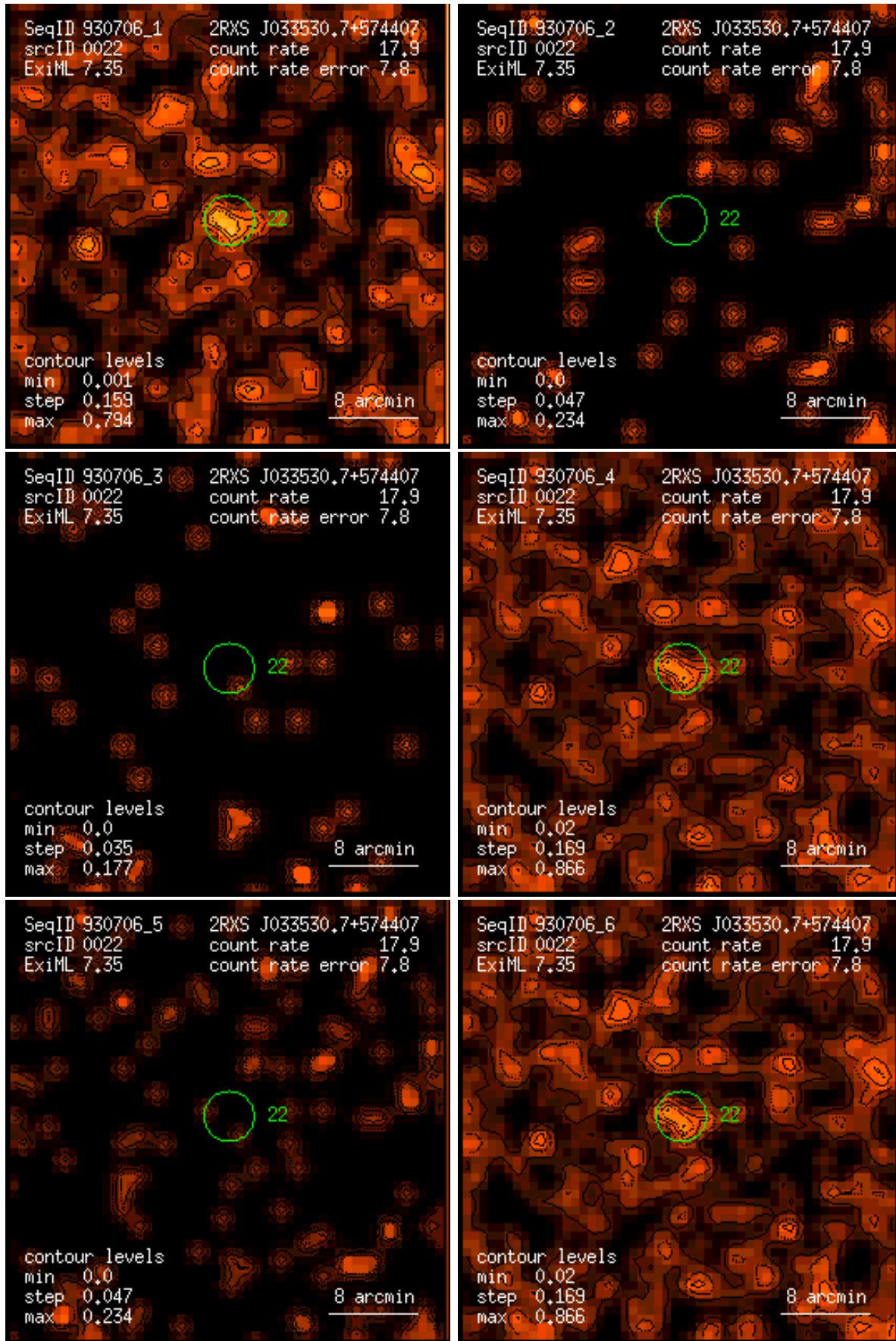
Figure 22: RASS 930706: detection 0022: band rate images, Gaussian filter: (1) PSPC channels 11 – 41, (2) 52 – 90, (3) 91 – 201, (4) 11 – 235, (5) 52 – 201, (6) 11 – 201. Broad band rates in counts/ks. Band rate contour levels in counts/ks/arcmin 2 .
