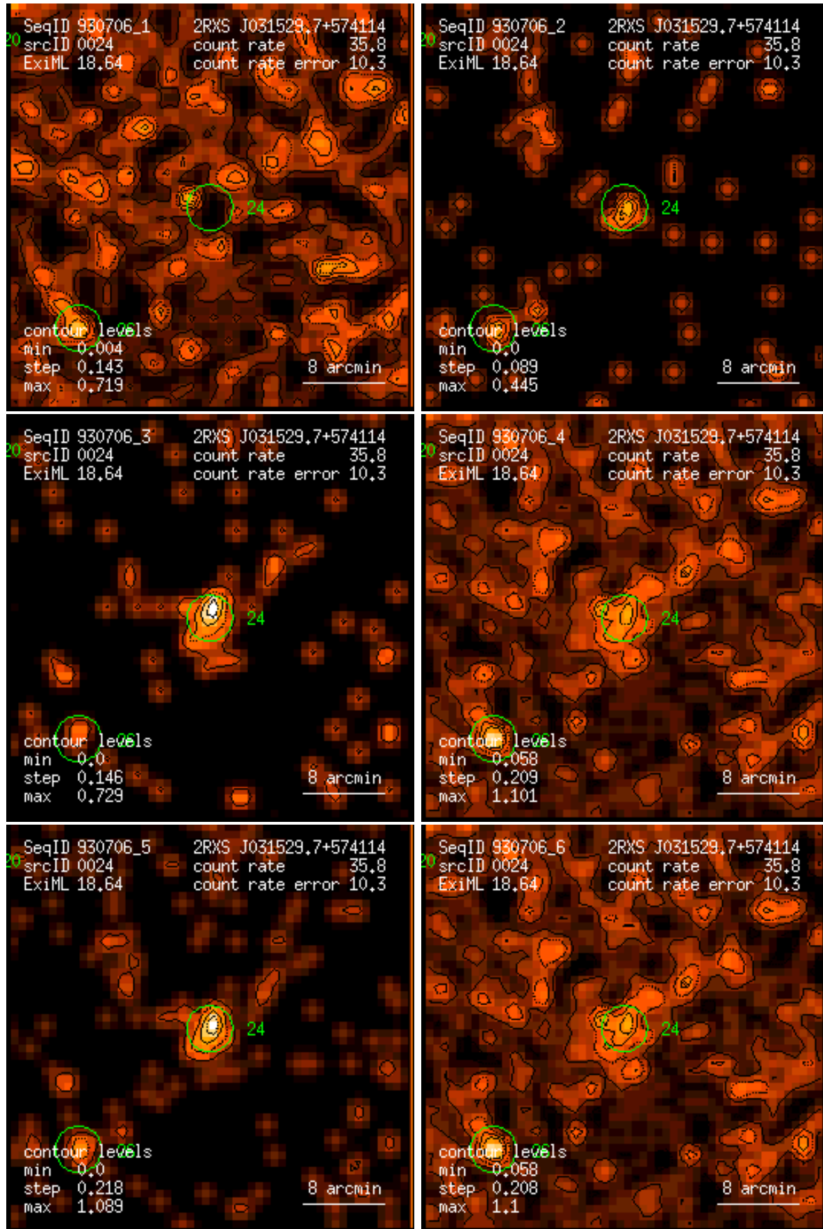
Figure 24: RASS 930706: detection 0024: band rate images, Gaussian filter: (1) PSPC channels 11 – 41, (2) 52 – 90, (3) 91 – 201, (4) 11 – 235, (5) 52 – 201, (6) 11 – 201. Broad band rates in counts/ks. Band rate contour levels in counts/ks/arcmin 2 .
