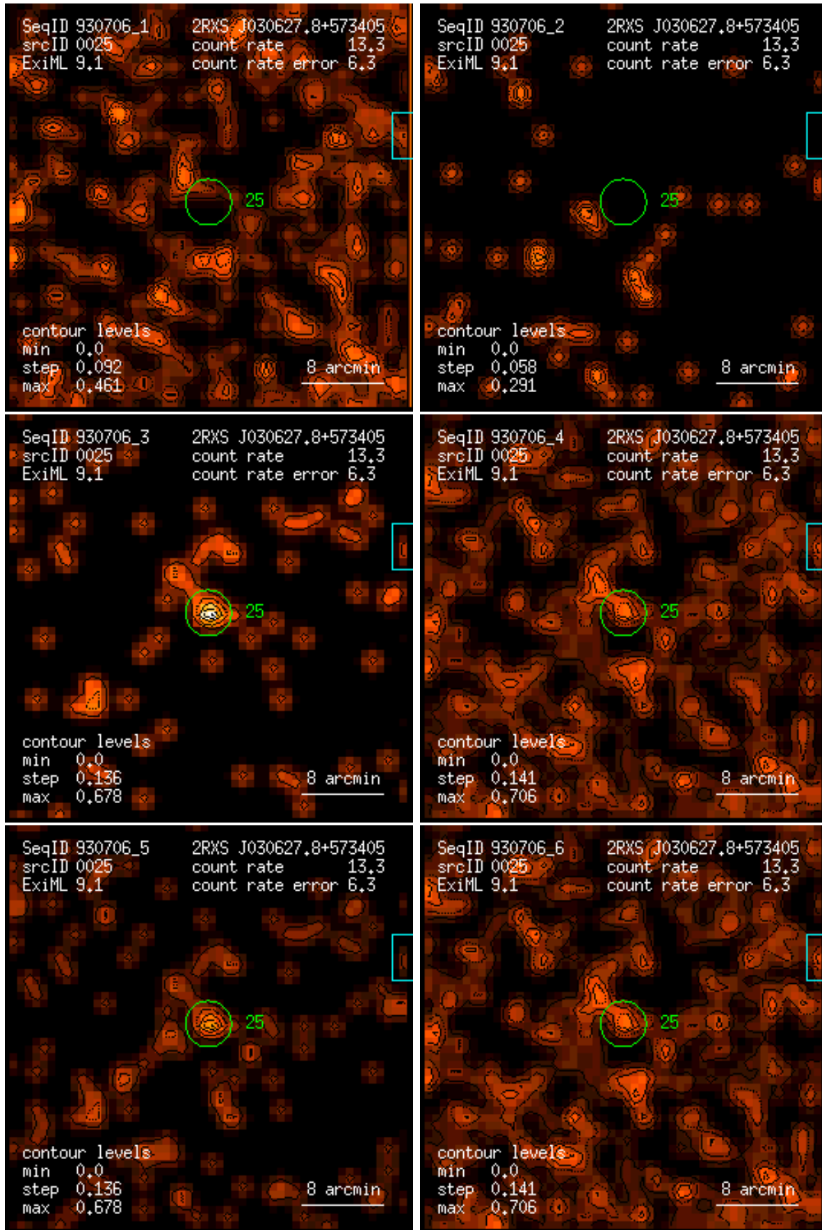
Figure 25: RASS 930706: detection 0025: band rate images, Gaussian filter: (1) PSPC channels 11 – 41, (2) 52 – 90, (3) 91 – 201, (4) 11 – 235, (5) 52 – 201, (6) 11 – 201. Broad band rates in counts/ks. Band rate contour levels in counts/ks/arcmin 2 .
