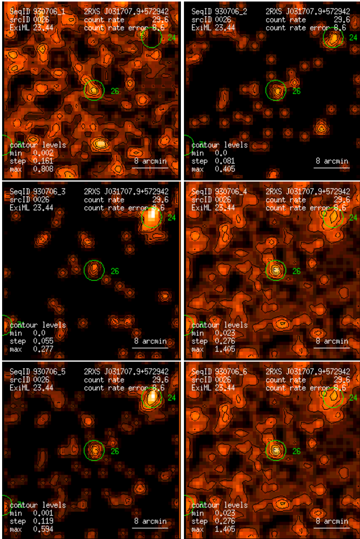
Figure 26: RASS 930706: detection 0026: band rate images, Gaussian filter: (1) PSPC channels 11 – 41, (2) 52 – 90, (3) 91 – 201, (4) 11 – 235, (5) 52 – 201, (6) 11 – 201. Broad band rates in counts/ks. Band rate contour levels in counts/ks/arcmin 2 .
