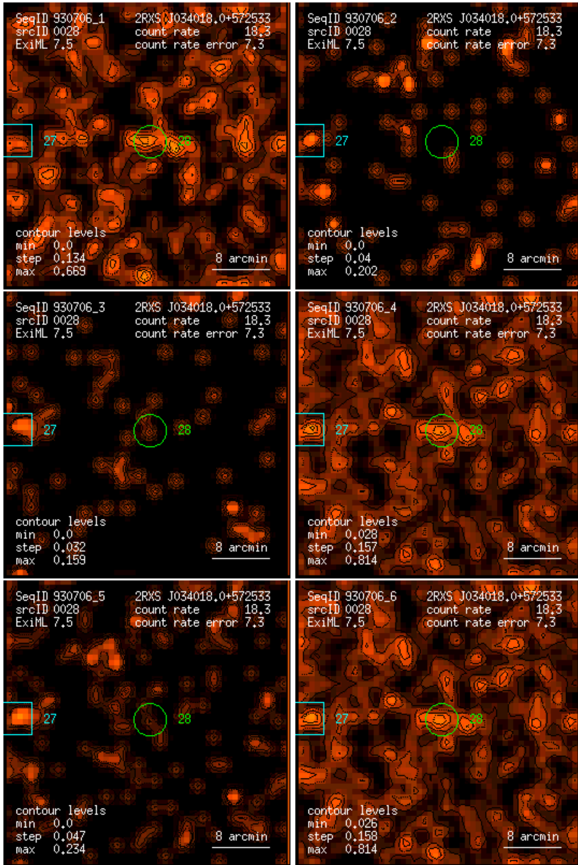
Figure 28: RASS 930706: detection 0028: band rate images, Gaussian filter: (1) PSPC channels 11 – 41, (2) 52 – 90, (3) 91 – 201, (4) 11 – 235, (5) 52 – 201, (6) 11 – 201. Broad band rates in counts/ks. Band rate contour levels in counts/ks/arcmin 2 .
