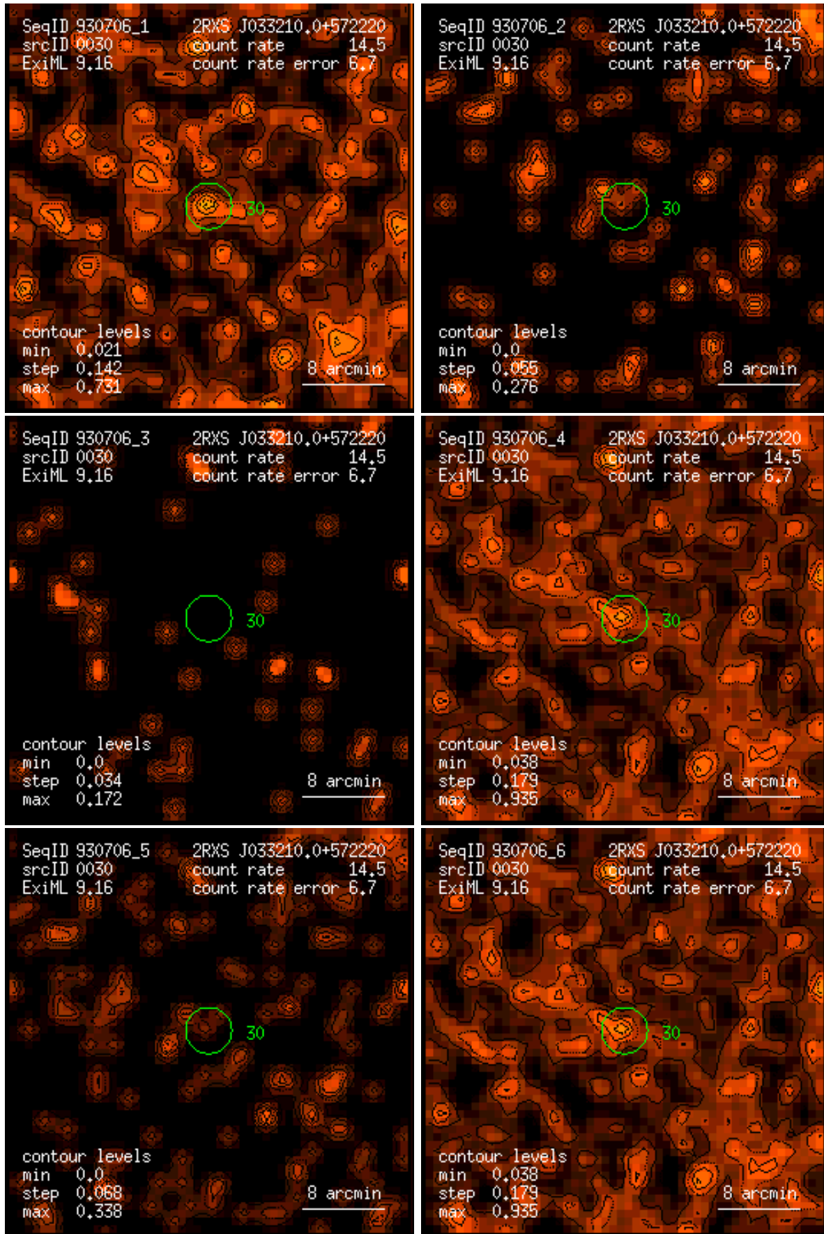
Figure 30: RASS 930706: detection 0030: band rate images, Gaussian filter: (1) PSPC channels 11 – 41, (2) 52 – 90, (3) 91 – 201, (4) 11 – 235, (5) 52 – 201, (6) 11 – 201. Broad band rates in counts/ks. Band rate contour levels in counts/ks/arcmin 2 .
