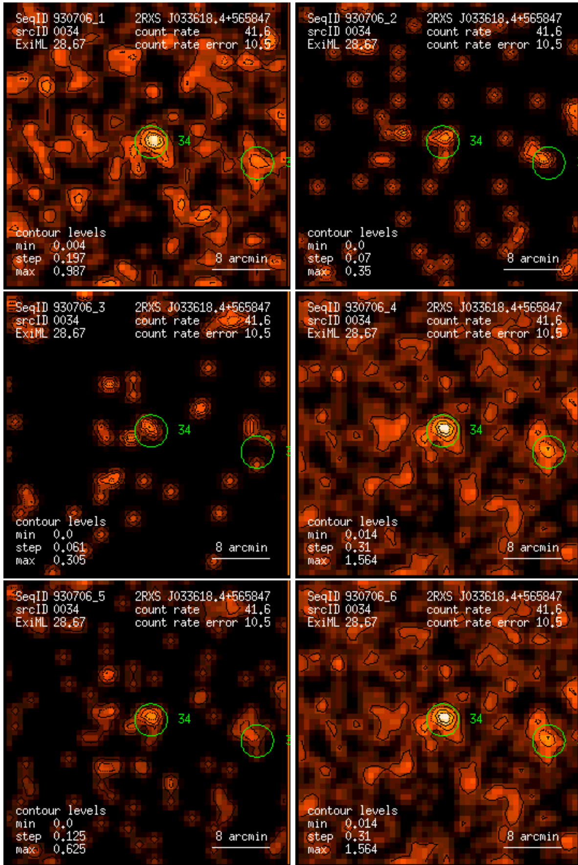
Figure 34: RASS 930706: detection 0034: band rate images, Gaussian filter: (1) PSPC channels 11 – 41, (2) 52 – 90, (3) 91 – 201, (4) 11 – 235, (5) 52 – 201, (6) 11 – 201. Broad band rates in counts/ks. Band rate contour levels in counts/ks/arcmin 2 .
