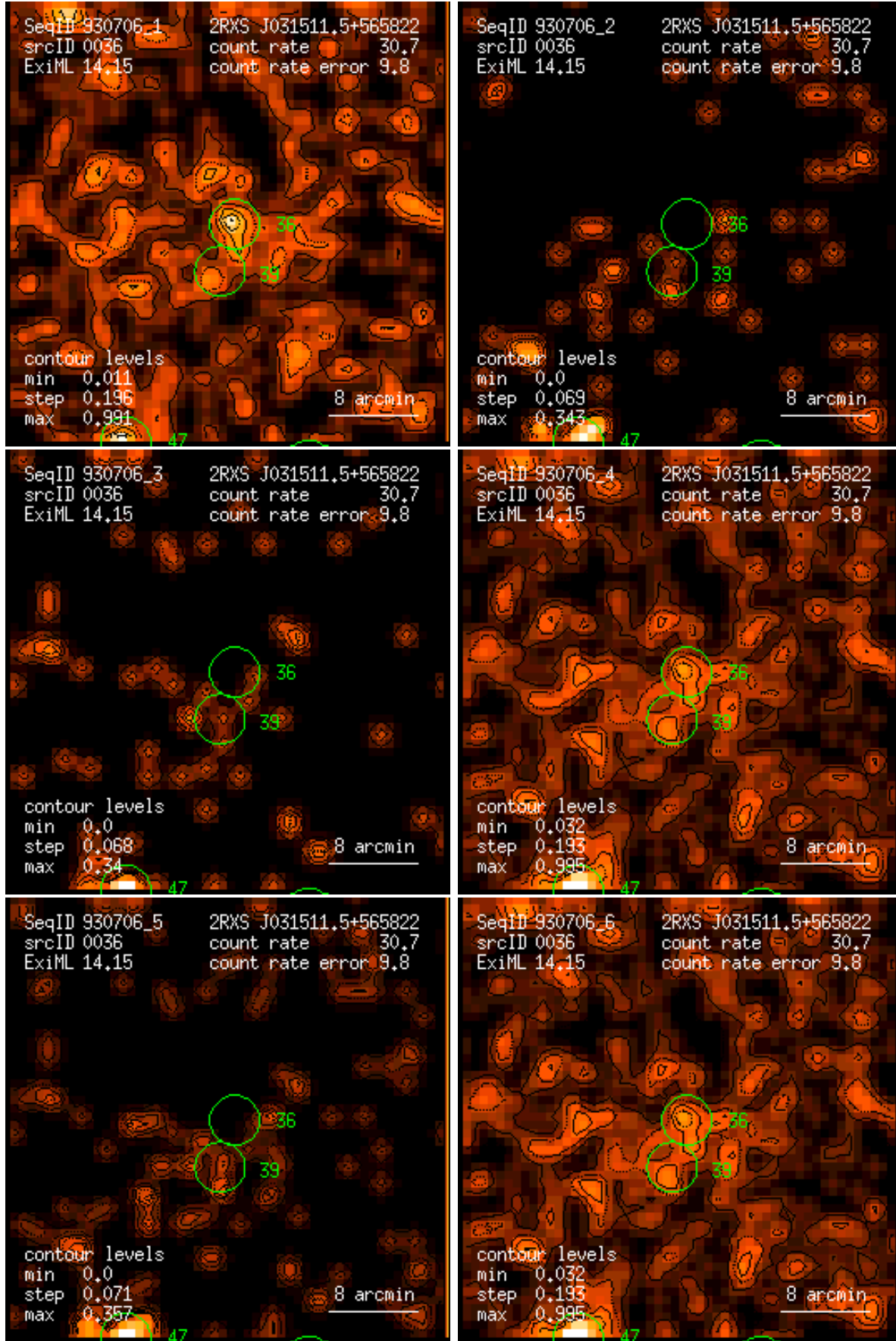
Figure 36: RASS 930706: detection 0036: band rate images, Gaussian filter: (1) PSPC channels 11 – 41, (2) 52 – 90, (3) 91 – 201, (4) 11 – 235, (5) 52 – 201, (6) 11 – 201. Broad band rates in counts/ks. Band rate contour levels in counts/ks/arcmin 2 .
