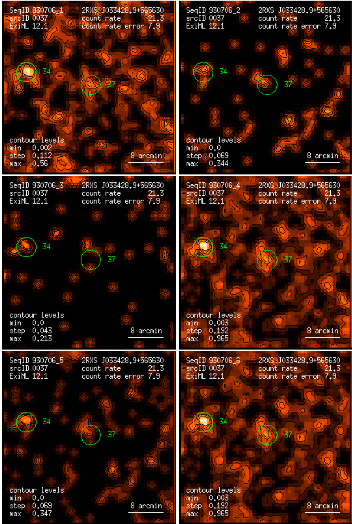
Figure 37: RASS 930706: detection 0037: band rate images, Gaussian filter: (1) PSPC channels 11 – 41, (2) 52 – 90, (3) 91 – 201, (4) 11 – 235, (5) 52 – 201, (6) 11 – 201. Broad band rates in counts/ks. Band rate contour levels in counts/ks/arcmin 2 .
