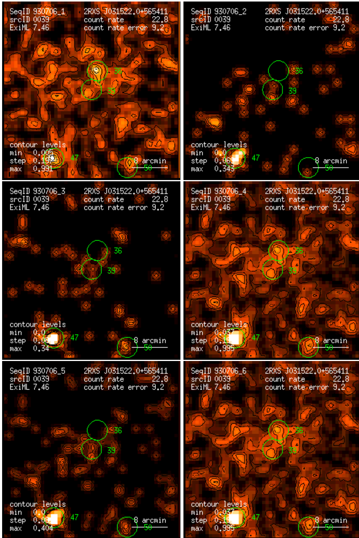
Figure 39: RASS 930706: detection 0039: band rate images, Gaussian filter: (1) PSPC channels 11 – 41, (2) 52 – 90, (3) 91 – 201, (4) 11 – 235, (5) 52 – 201, (6) 11 – 201. Broad band rates in counts/ks. Band rate contour levels in counts/ks/arcmin 2 .
