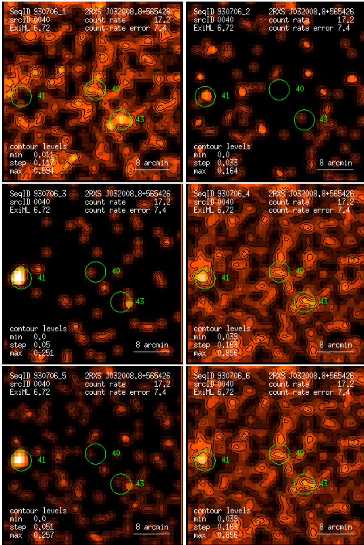
Figure 40: RASS 930706: detection 0040: band rate images, Gaussian filter: (1) PSPC channels 11 – 41, (2) 52 – 90, (3) 91 – 201, (4) 11 – 235, (5) 52 – 201, (6) 11 – 201. Broad band rates in counts/ks. Band rate contour levels in counts/ks/arcmin 2 .
