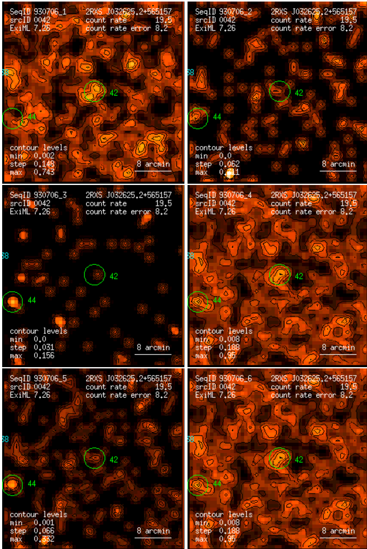
Figure 42: RASS 930706: detection 0042: band rate images, Gaussian filter: (1) PSPC channels 11 – 41, (2) 52 – 90, (3) 91 – 201, (4) 11 – 235, (5) 52 – 201, (6) 11 – 201. Broad band rates in counts/ks. Band rate contour levels in counts/ks/arcmin 2 .
