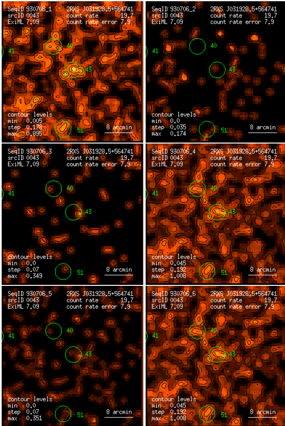
Figure 43: RASS 930706: detection 0043: band rate images, Gaussian filter: (1) PSPC channels 11 – 41, (2) 52 – 90, (3) 91 – 201, (4) 11 – 235, (5) 52 – 201, (6) 11 – 201. Broad band rates in counts/ks. Band rate contour levels in counts/ks/arcmin 2 .
