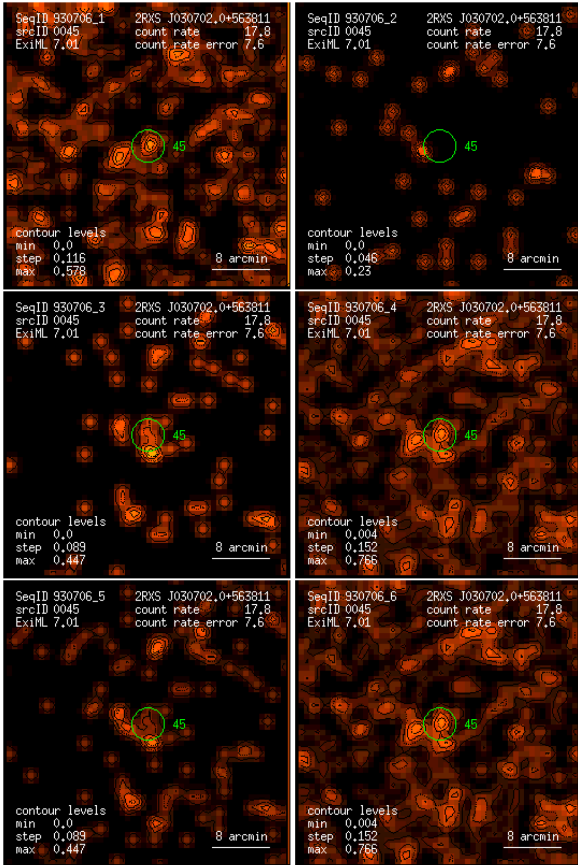
Figure 45: RASS 930706: detection 0045: band rate images, Gaussian filter: (1) PSPC channels 11 – 41, (2) 52 – 90, (3) 91 – 201, (4) 11 – 235, (5) 52 – 201, (6) 11 – 201. Broad band rates in counts/ks. Band rate contour levels in counts/ks/arcmin 2 .
