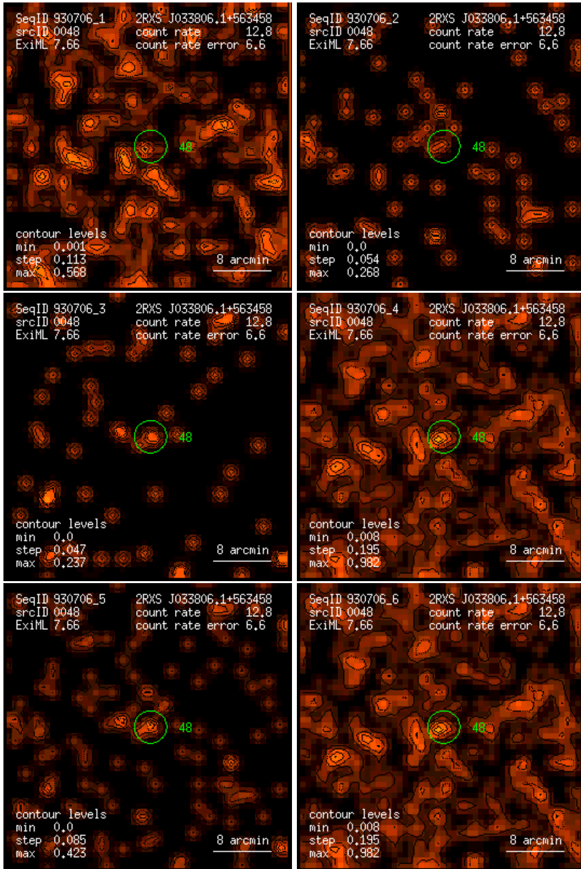
Figure 48: RASS 930706: detection 0048: band rate images, Gaussian filter: (1) PSPC channels 11 – 41, (2) 52 – 90, (3) 91 – 201, (4) 11 – 235, (5) 52 – 201, (6) 11 – 201. Broad band rates in counts/ks. Band rate contour levels in counts/ks/arcmin 2 .
