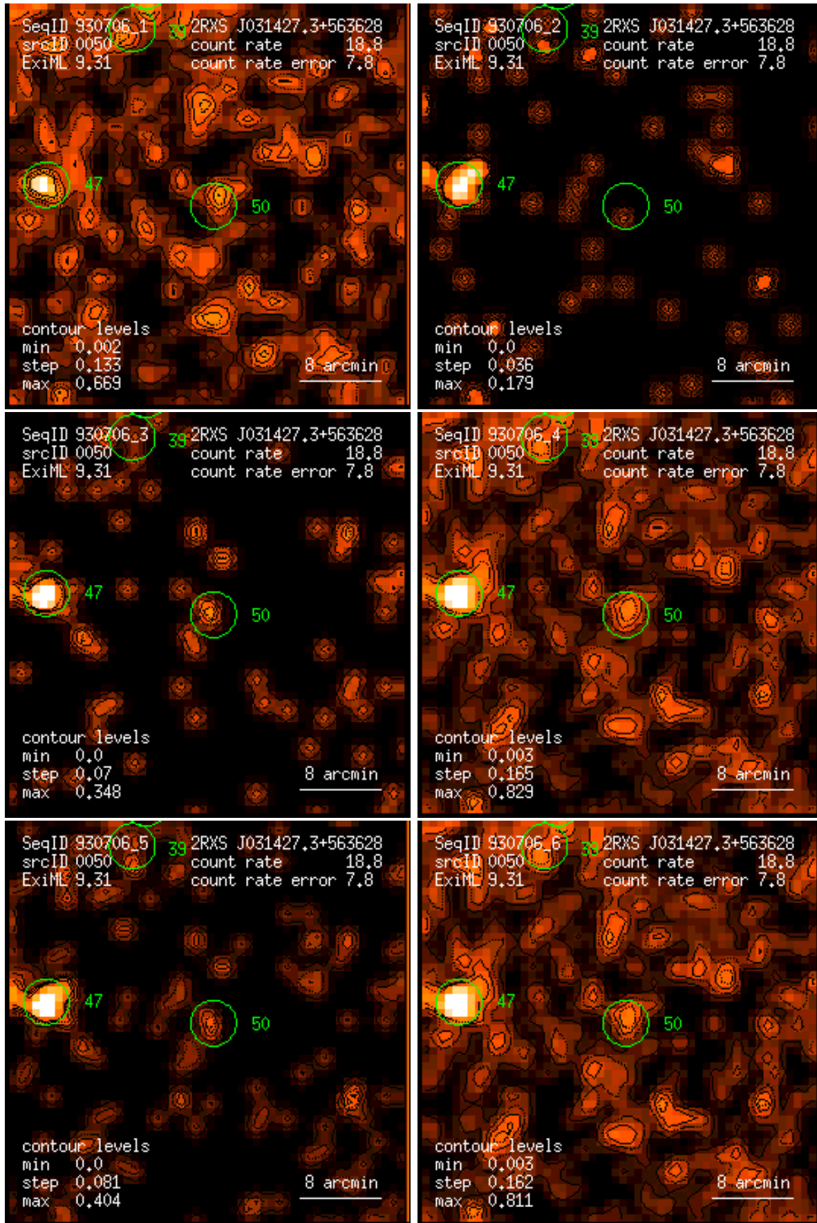
Figure 50: RASS 930706: detection 0050: band rate images, Gaussian filter: (1) PSPC channels 11 – 41, (2) 52 – 90, (3) 91 – 201, (4) 11 – 235, (5) 52 – 201, (6) 11 – 201. Broad band rates in counts/ks. Band rate contour levels in counts/ks/arcmin 2 .
