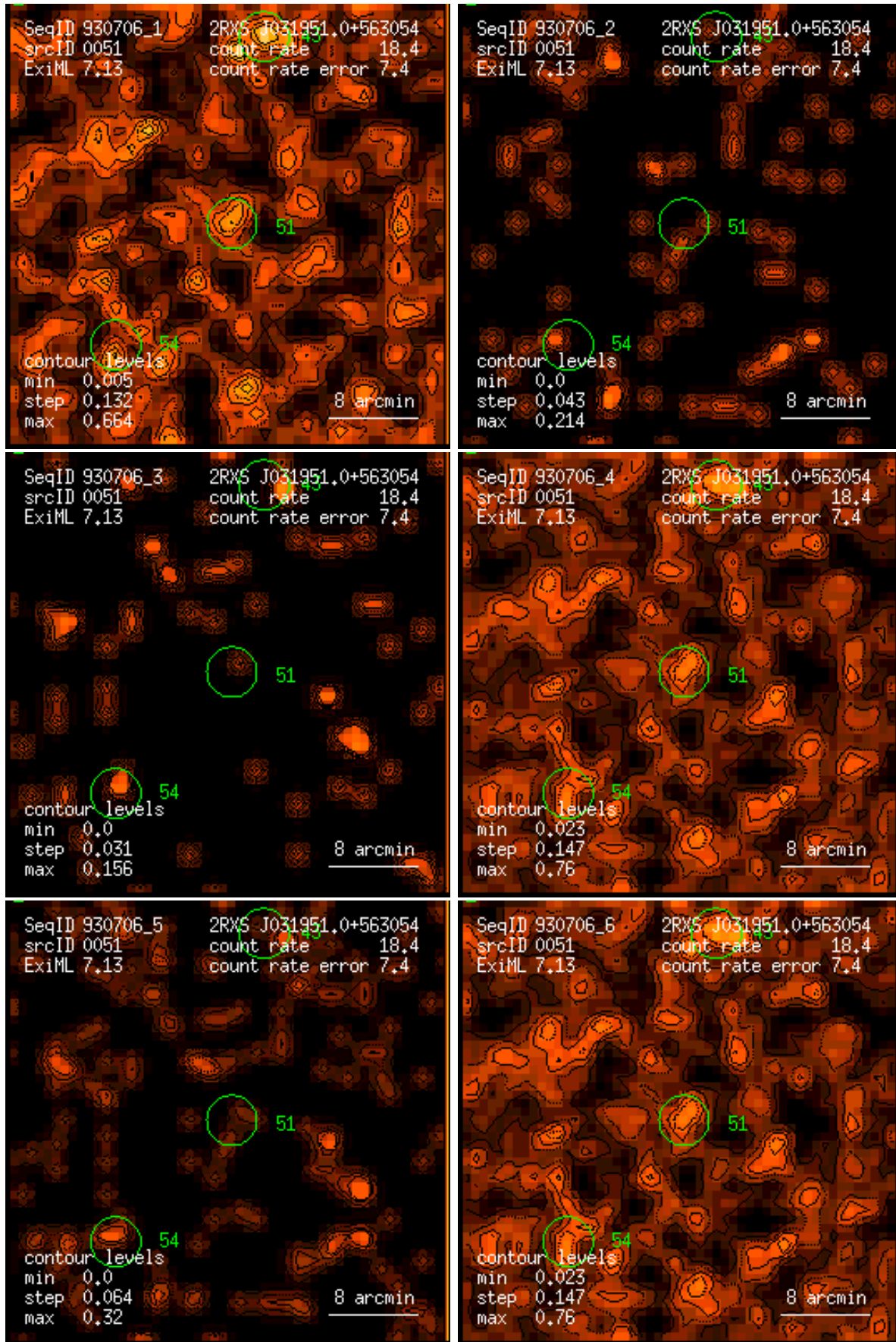
Figure 51: RASS 930706: detection 0051: band rate images, Gaussian filter: (1) PSPC channels 11 – 41, (2) 52 – 90, (3) 91 – 201, (4) 11 – 235, (5) 52 – 201, (6) 11 – 201. Broad band rates in counts/ks. Band rate contour levels in counts/ks/arcmin 2 .
