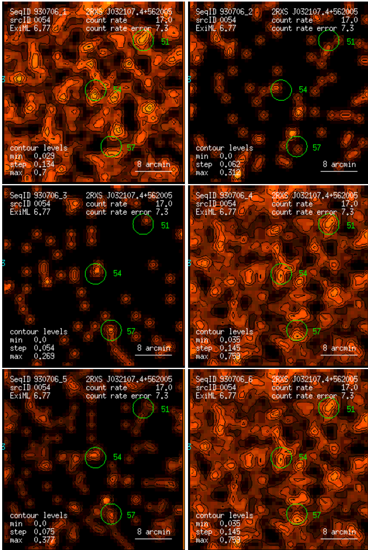
Figure 54: RASS 930706: detection 0054: band rate images, Gaussian filter: (1) PSPC channels 11 – 41, (2) 52 – 90, (3) 91 – 201, (4) 11 – 235, (5) 52 – 201, (6) 11 – 201. Broad band rates in counts/ks. Band rate contour levels in counts/ks/arcmin 2 .
