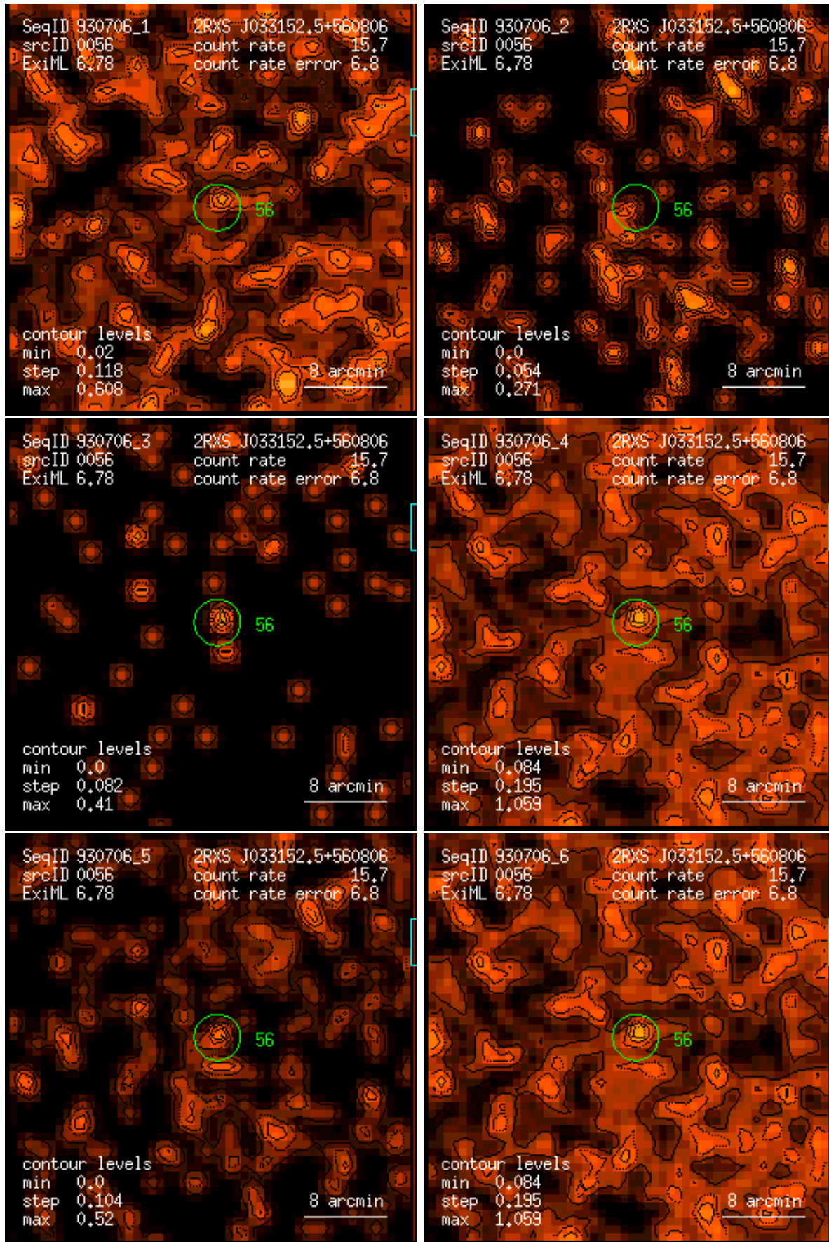
Figure 56: RASS 930706: detection 0056: band rate images, Gaussian filter: (1) PSPC channels 11 – 41, (2) 52 – 90, (3) 91 – 201, (4) 11 – 235, (5) 52 – 201, (6) 11 – 201. Broad band rates in counts/ks. Band rate contour levels in counts/ks/arcmin 2 .
