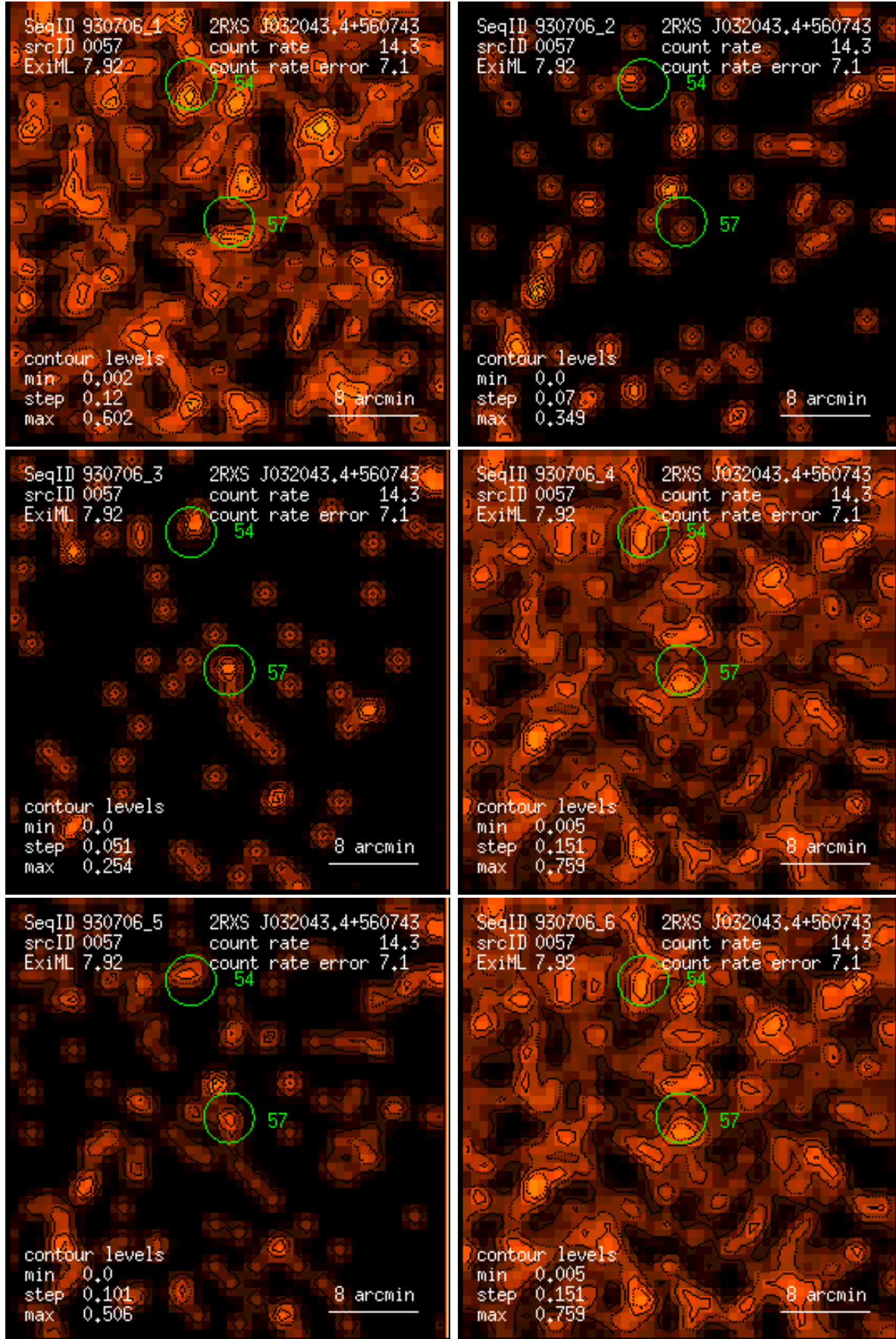
Figure 57: RASS 930706: detection 0057: band rate images, Gaussian filter: (1) PSPC channels 11 – 41, (2) 52 – 90, (3) 91 – 201, (4) 11 – 235, (5) 52 – 201, (6) 11 – 201. Broad band rates in counts/ks. Band rate contour levels in counts/ks/arcmin 2 .
