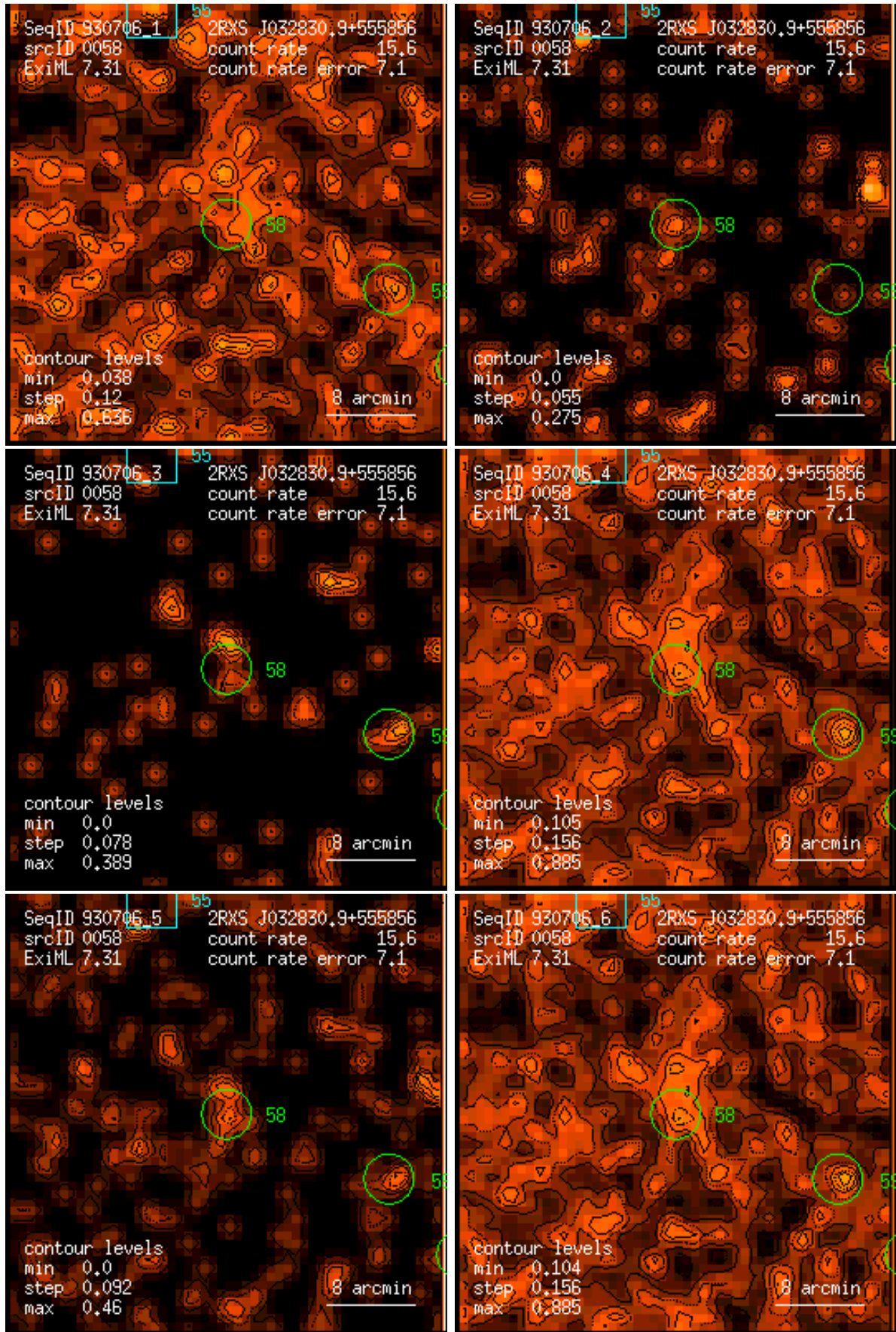
Figure 58: RASS 930706: detection 0058: band rate images, Gaussian filter: (1) PSPC channels 11 – 41, (2) 52 – 90, (3) 91 – 201, (4) 11 – 235, (5) 52 – 201, (6) 11 – 201. Broad band rates in counts/ks. Band rate contour levels in counts/ks/arcmin 2 .
