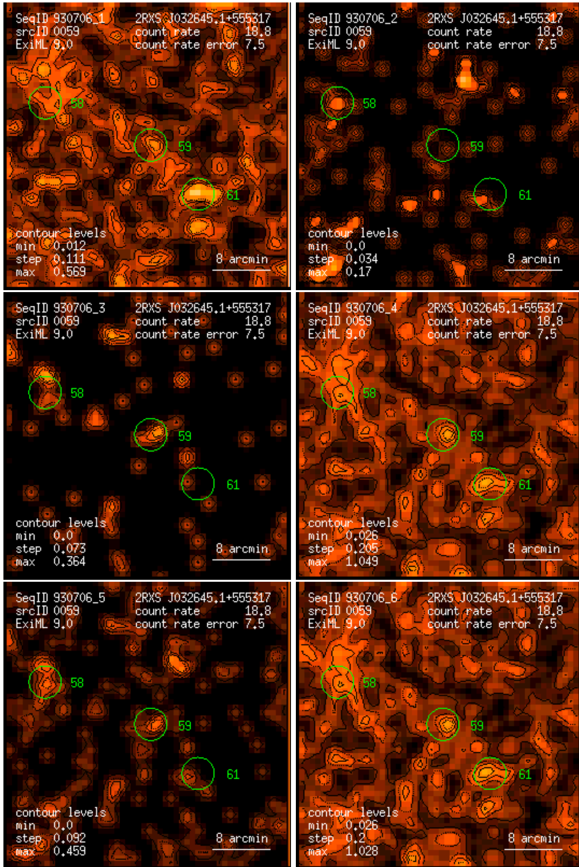
Figure 59: RASS 930706: detection 0059: band rate images, Gaussian filter: (1) PSPC channels 11 – 41, (2) 52 – 90, (3) 91 – 201, (4) 11 – 235, (5) 52 – 201, (6) 11 – 201. Broad band rates in counts/ks. Band rate contour levels in counts/ks/arcmin 2 .
