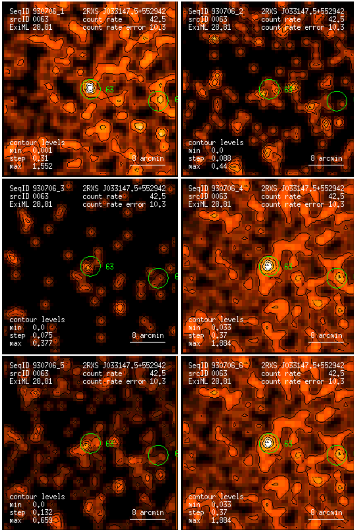
Figure 63: RASS 930706: detection 0063: band rate images, Gaussian filter: (1) PSPC channels 11 – 41, (2) 52 – 90, (3) 91 – 201, (4) 11 – 235, (5) 52 – 201, (6) 11 – 201. Broad band rates in counts/ks. Band rate contour levels in counts/ks/arcmin 2 .
