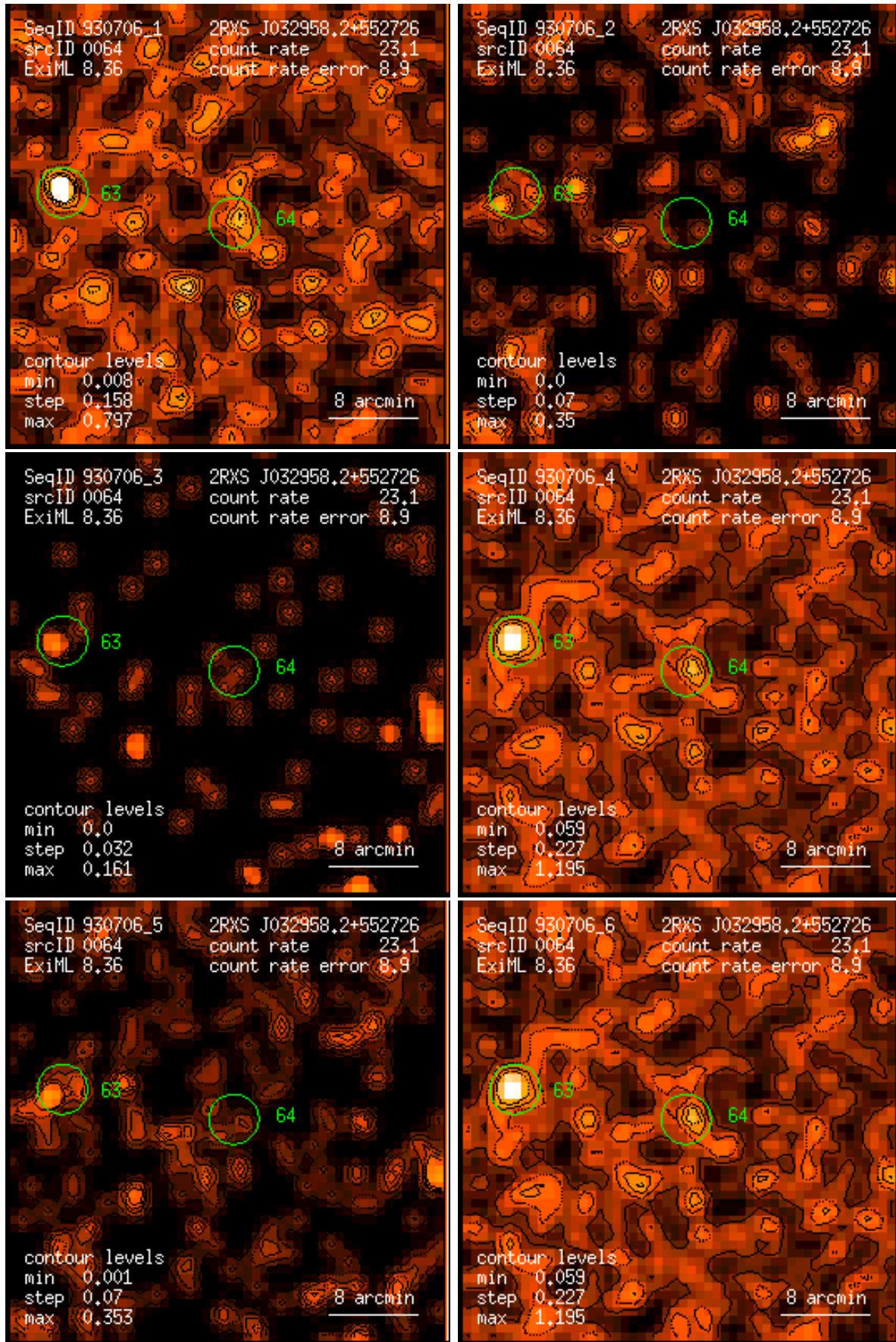
Figure 64: RASS 930706: detection 0064: band rate images, Gaussian filter: (1) PSPC channels 11 – 41, (2) 52 – 90, (3) 91 – 201, (4) 11 – 235, (5) 52 – 201, (6) 11 – 201. Broad band rates in counts/ks. Band rate contour levels in counts/ks/arcmin 2 .
