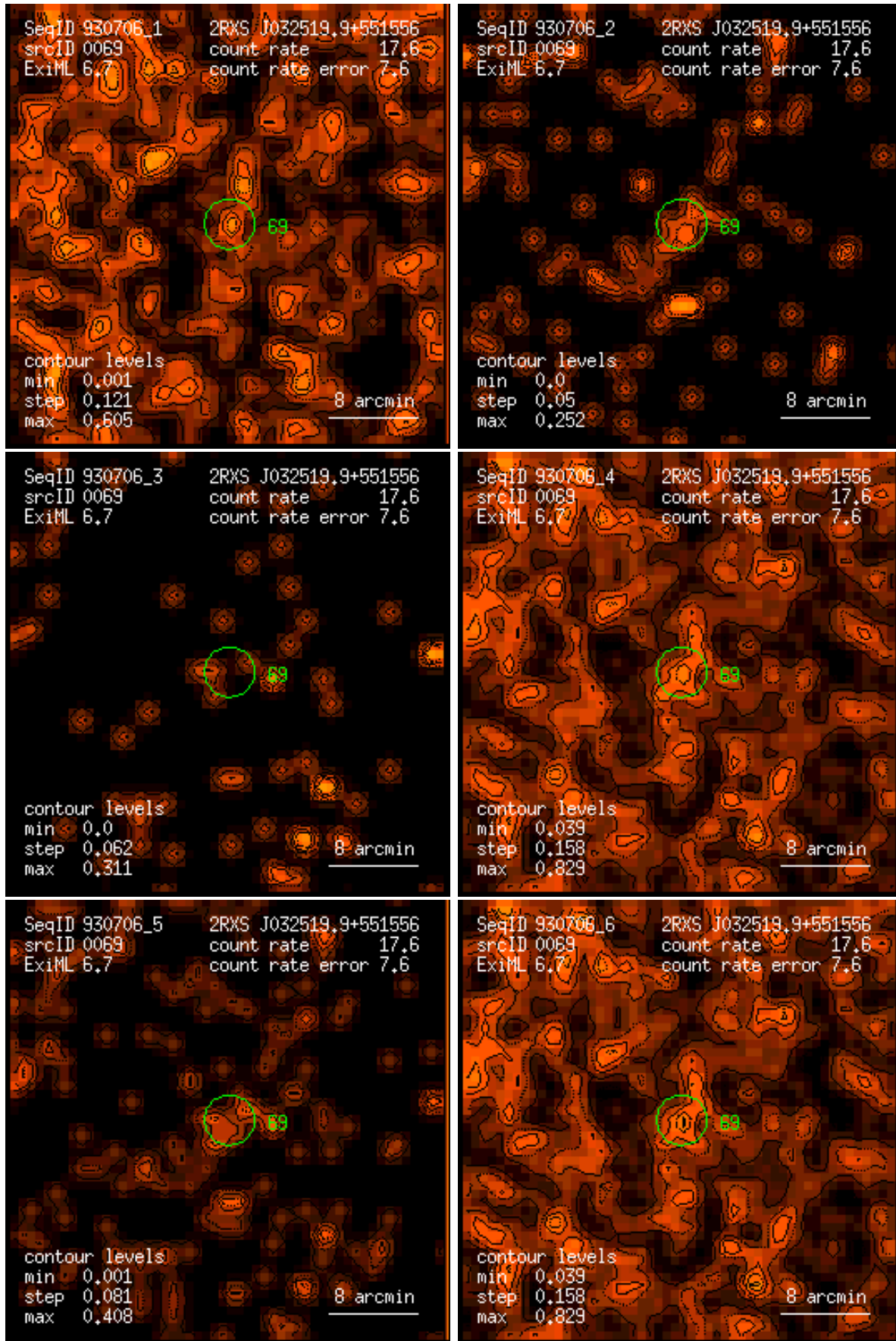
Figure 69: RASS 930706: detection 0069: band rate images, Gaussian filter: (1) PSPC channels 11 – 41, (2) 52 – 90, (3) 91 – 201, (4) 11 – 235, (5) 52 – 201, (6) 11 – 201. Broad band rates in counts/ks. Band rate contour levels in counts/ks/arcmin 2 .
