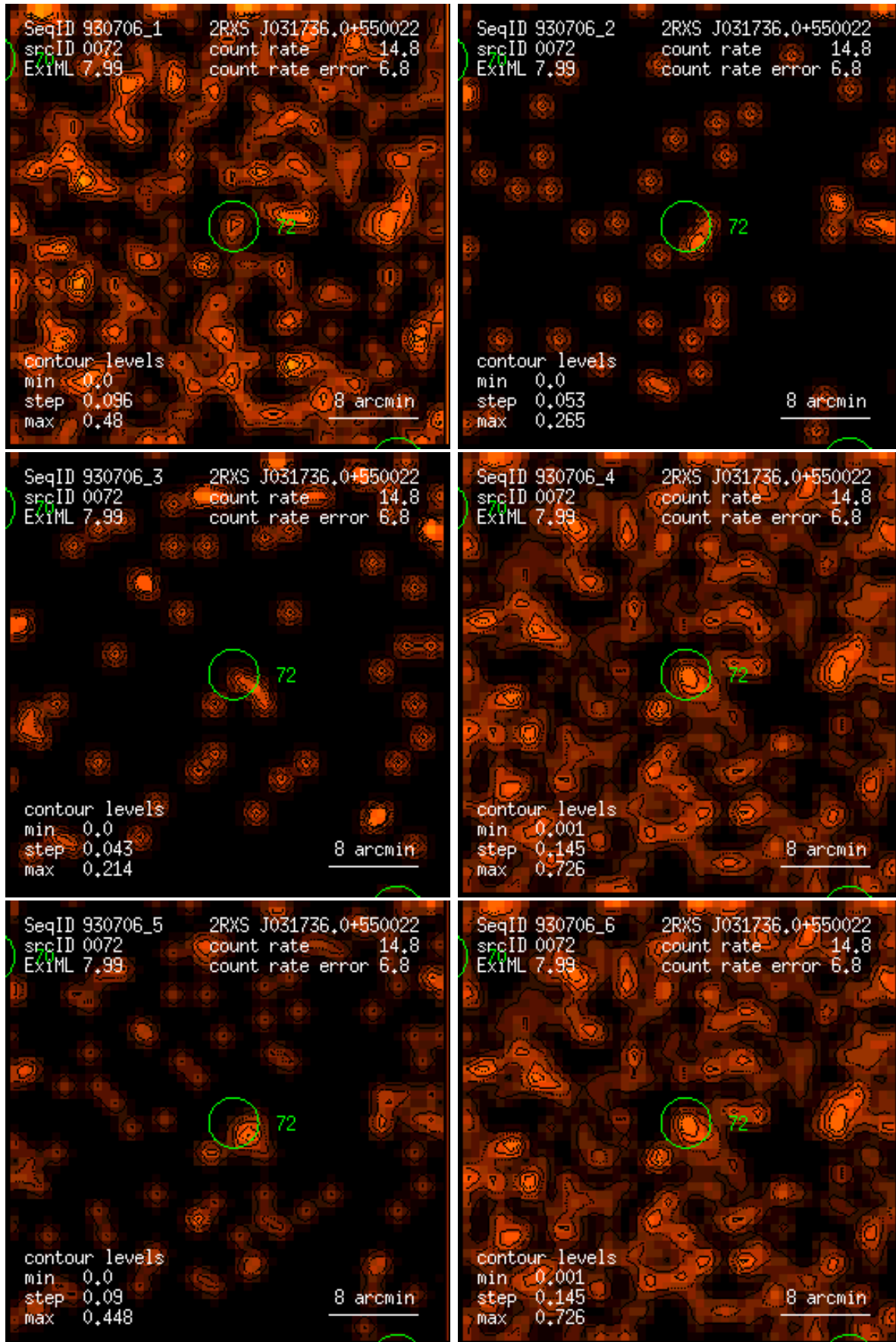
Figure 72: RASS 930706: detection 0072: band rate images, Gaussian filter: (1) PSPC channels 11 – 41, (2) 52 – 90, (3) 91 – 201, (4) 11 – 235, (5) 52 – 201, (6) 11 – 201. Broad band rates in counts/ks. Band rate contour levels in counts/ks/arcmin 2 .
