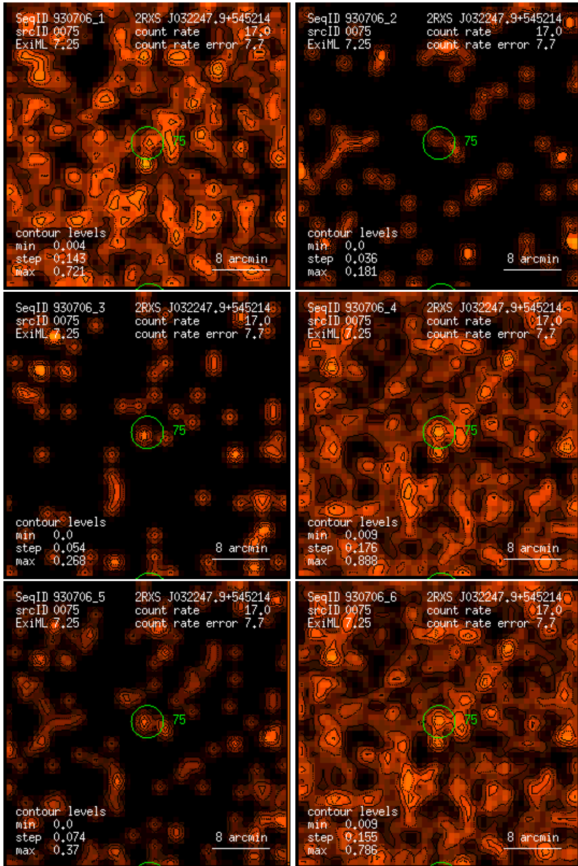
Figure 75: RASS 930706: detection 0075: band rate images, Gaussian filter: (1) PSPC channels 11 – 41, (2) 52 – 90, (3) 91 – 201, (4) 11 – 235, (5) 52 – 201, (6) 11 – 201. Broad band rates in counts/ks. Band rate contour levels in counts/ks/arcmin 2 .
